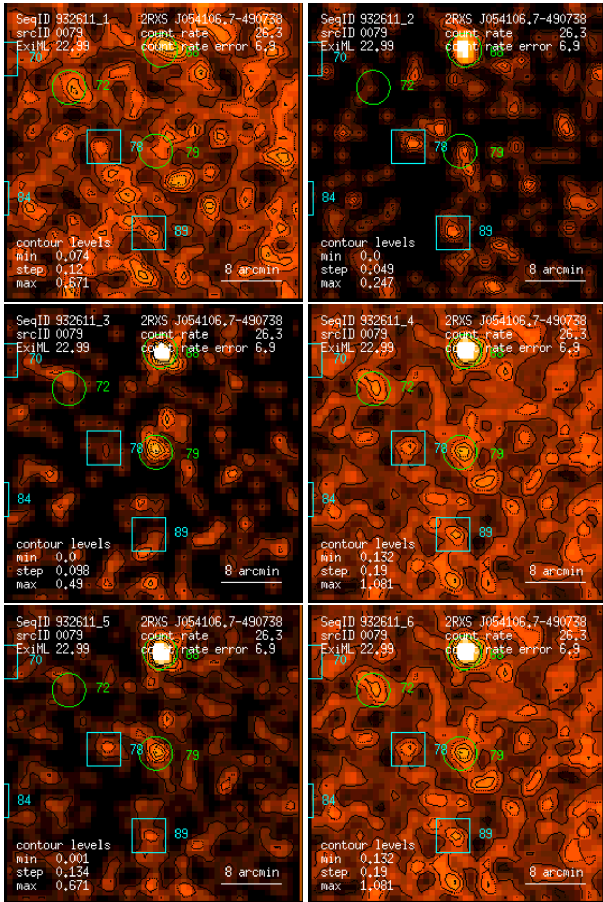
Figure 79: RASS 932611: detection 0079: band rate images, Gaussian filter: (1) PSPC channels 11 – 41, (2) 52 – 90, (3) 91 – 201, (4) 11 – 235, (5) 52 – 201, (6) 11 – 201. Broad band rates in counts/ks. Band rate contour levels in counts/ks/arcmin 2 .
