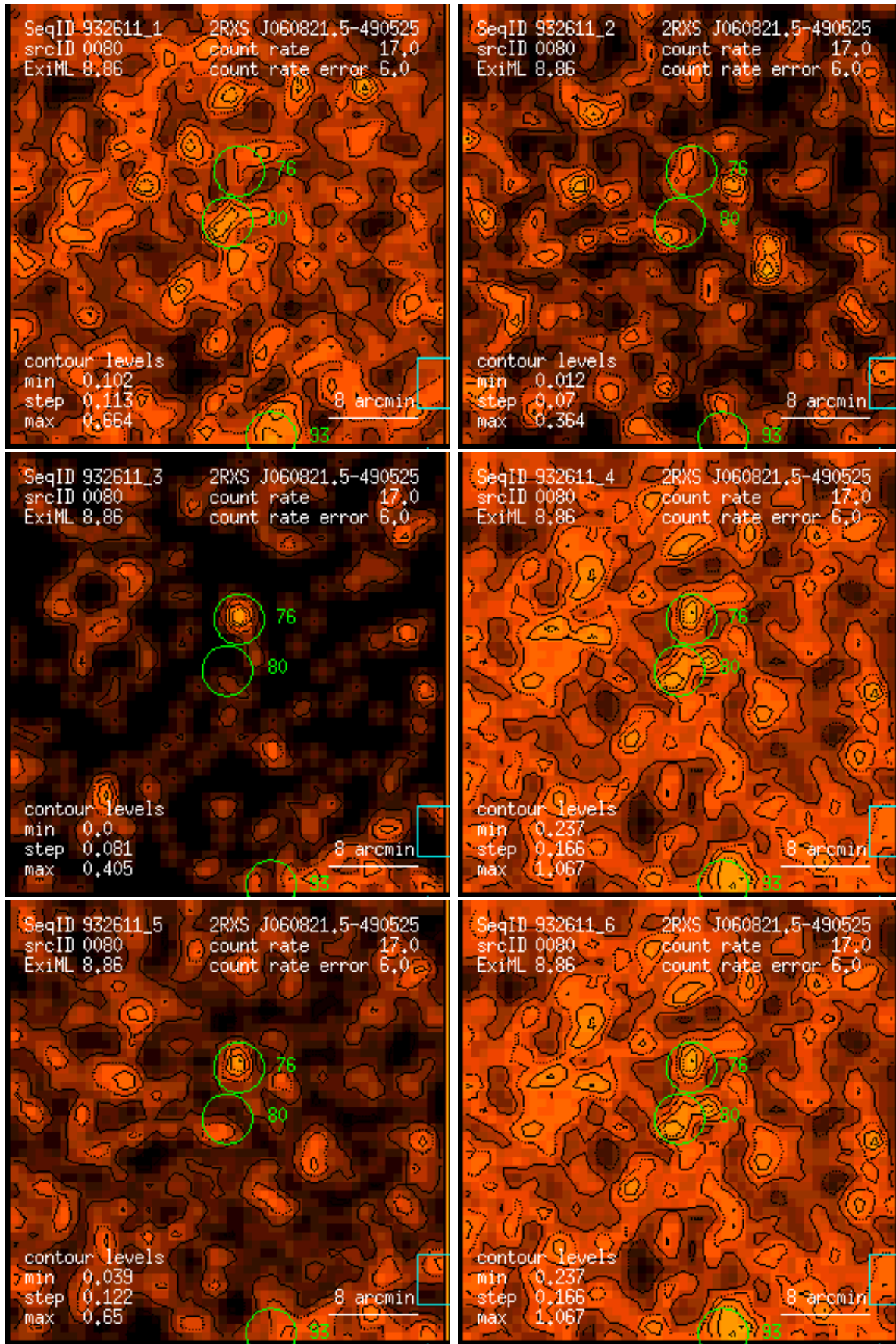
Figure 80: RASS 932611: detection 0080: band rate images, Gaussian filter: (1) PSPC channels 11 – 41, (2) 52 – 90, (3) 91 – 201, (4) 11 – 235, (5) 52 – 201, (6) 11 – 201. Broad band rates in counts/ks. Band rate contour levels in counts/ks/arcmin 2 .
