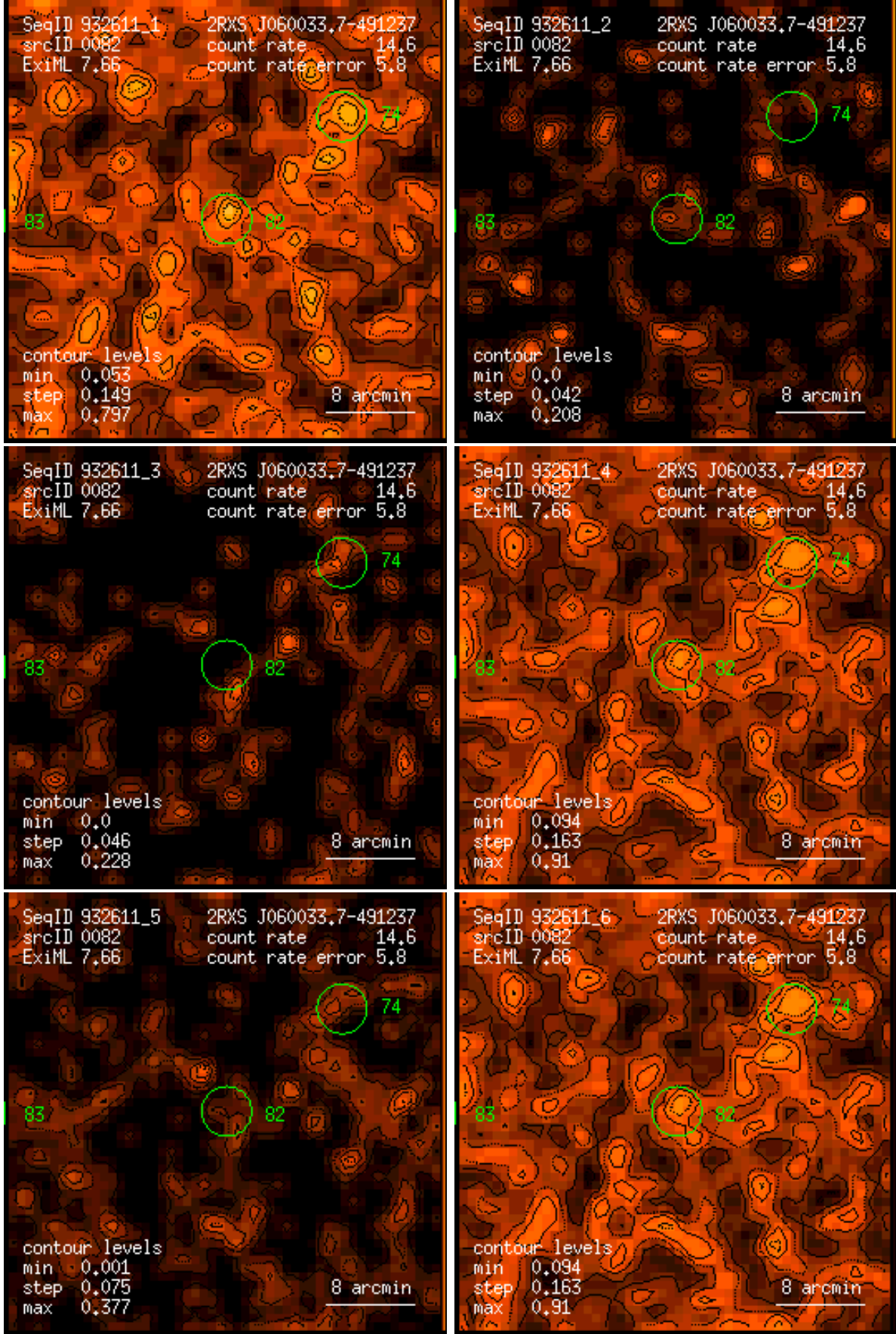
Figure 82: RASS 932611: detection 0082: band rate images, Gaussian filter: (1) PSPC channels 11 – 41, (2) 52 – 90, (3) 91 – 201, (4) 11 – 235, (5) 52 – 201, (6) 11 – 201. Broad band rates in counts/ks. Band rate contour levels in counts/ks/arcmin 2 .
