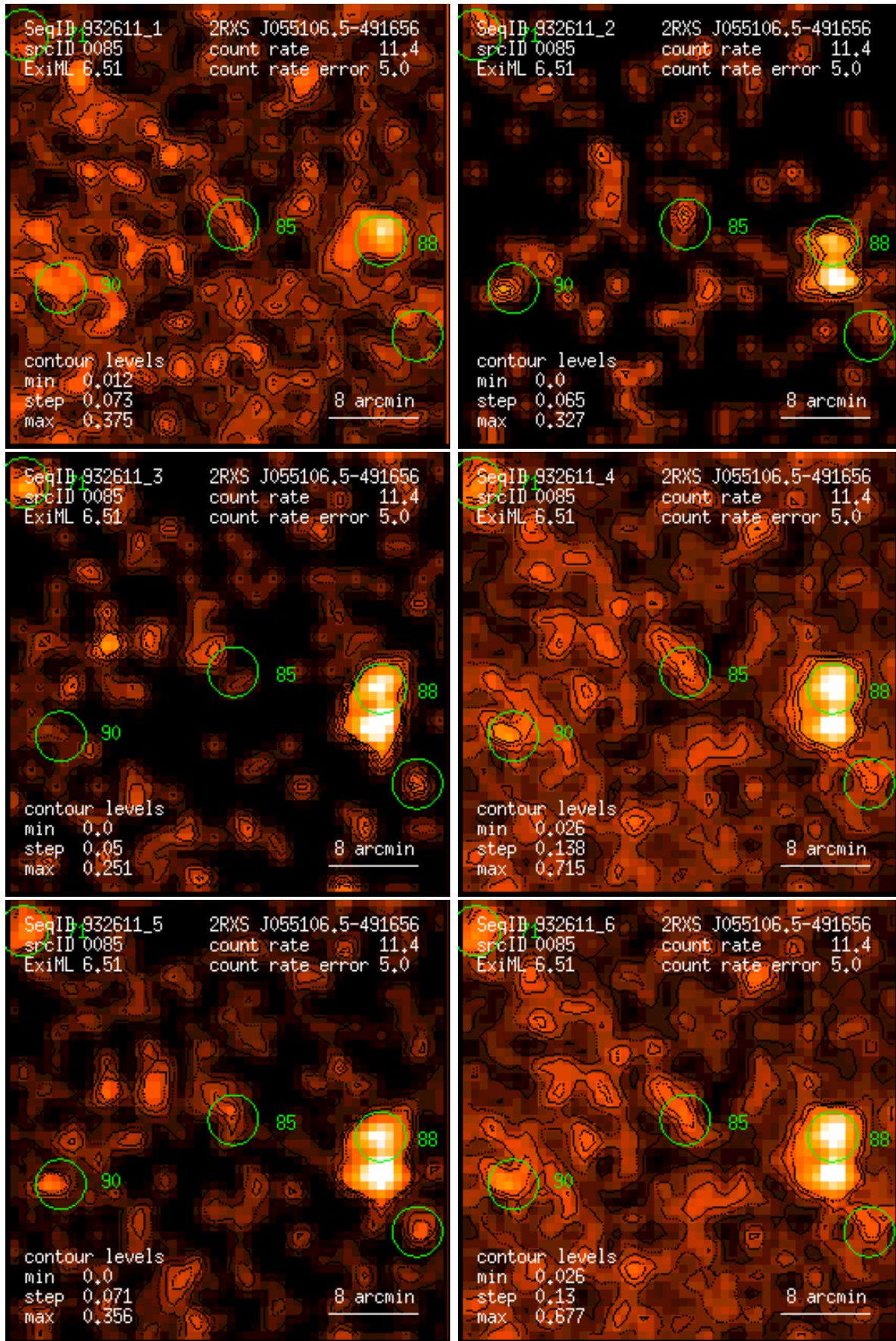
Figure 85: RASS 932611: detection 0085: band rate images, Gaussian filter: (1) PSPC channels 11 – 41, (2) 52 – 90, (3) 91 – 201, (4) 11 – 235, (5) 52 – 201, (6) 11 – 201. Broad band rates in counts/ks. Band rate contour levels in counts/ks/arcmin 2 .
