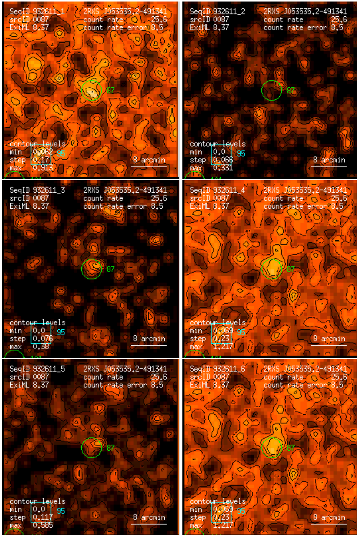
Figure 87: RASS 932611: detection 0087: band rate images, Gaussian filter: (1) PSPC channels 11 – 41, (2) 52 – 90, (3) 91 – 201, (4) 11 – 235, (5) 52 – 201, (6) 11 – 201. Broad band rates in counts/ks. Band rate contour levels in counts/ks/arcmin 2 .
