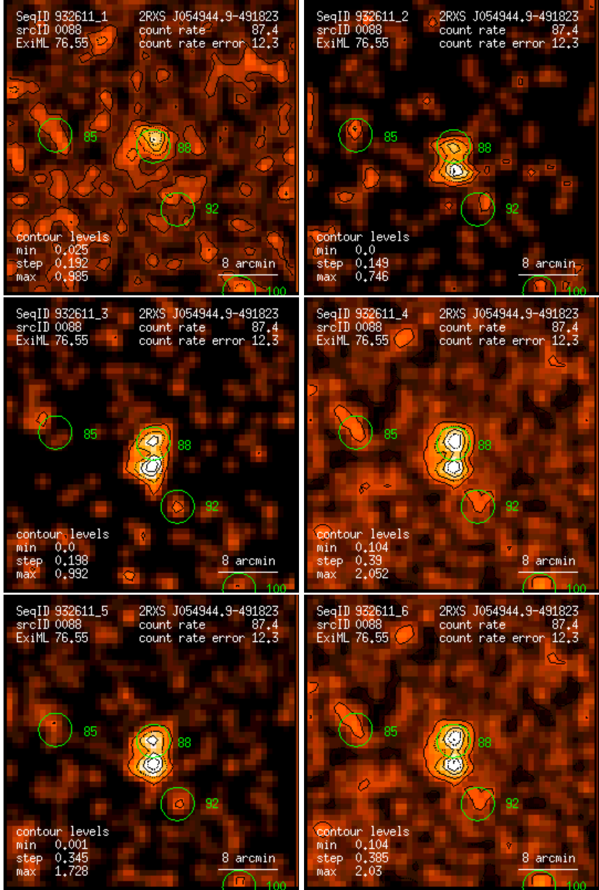
Figure 88: RASS 932611: detection 0088: band rate images, Gaussian filter: (1) PSPC channels 11 – 41, (2) 52 – 90, (3) 91 – 201, (4) 11 – 235, (5) 52 – 201, (6) 11 – 201. Broad band rates in counts/ks. Band rate contour levels in counts/ks/arcmin 2 .
