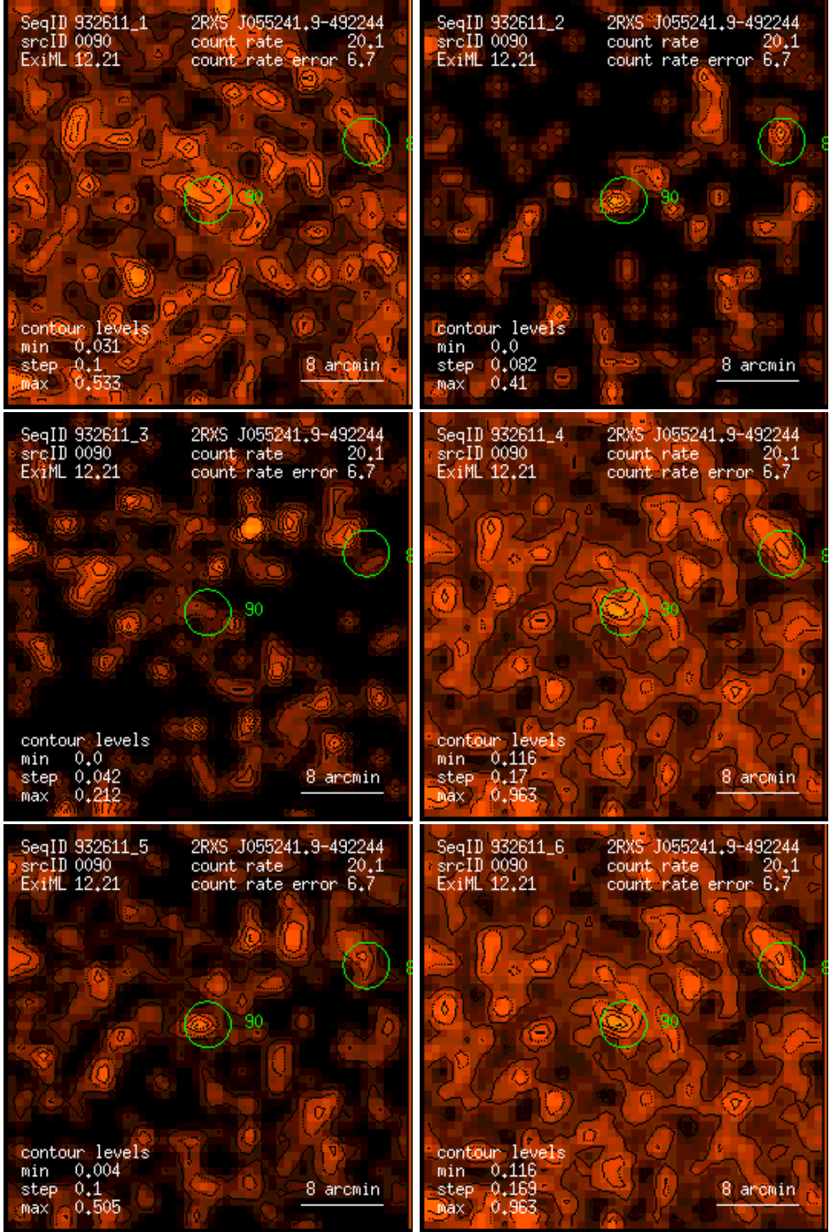
Figure 90: RASS 932611: detection 0090: band rate images, Gaussian filter: (1) PSPC channels 11 – 41, (2) 52 – 90, (3) 91 – 201, (4) 11 – 235, (5) 52 – 201, (6) 11 – 201. Broad band rates in counts/ks. Band rate contour levels in counts/ks/arcmin 2 .
