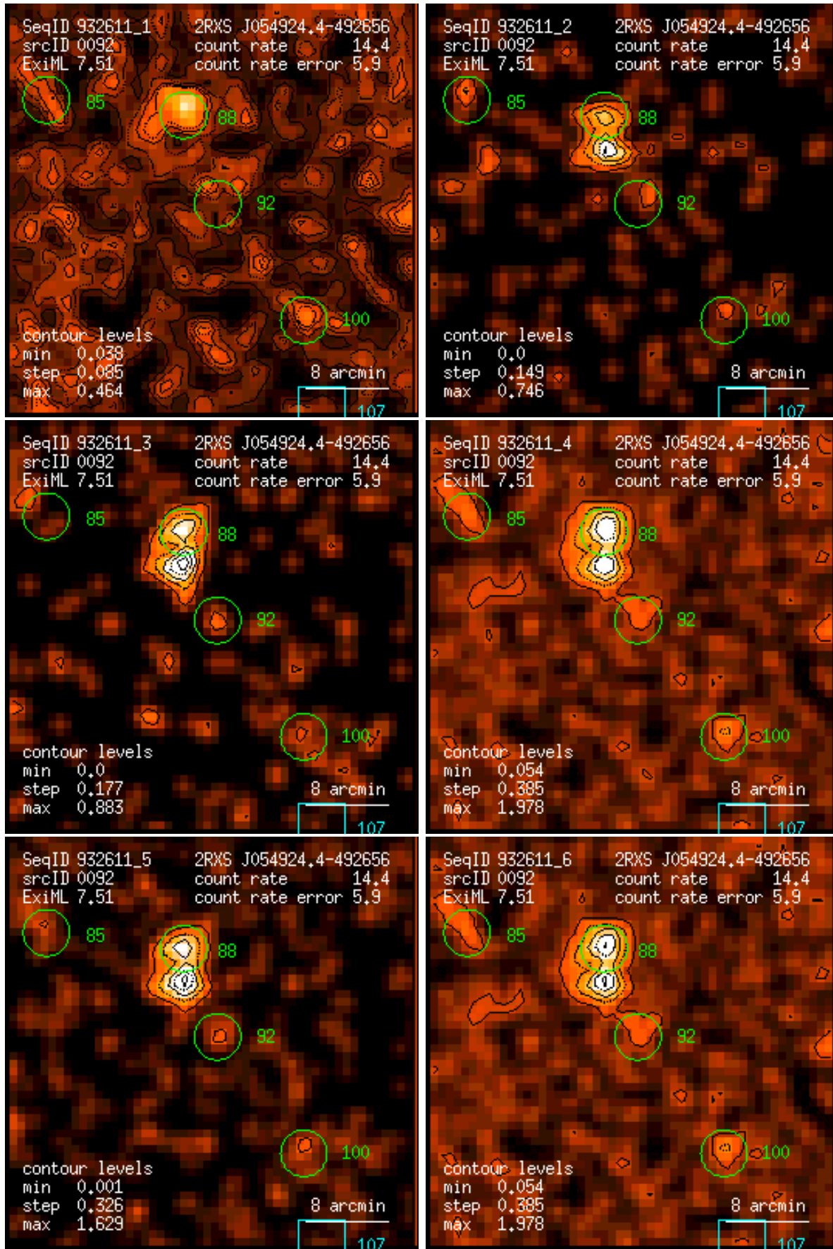
Figure 92: RASS 932611: detection 0092: band rate images, Gaussian filter: (1) PSPC channels 11 – 41, (2) 52 – 90, (3) 91 – 201, (4) 11 – 235, (5) 52 – 201, (6) 11 – 201. Broad band rates in counts/ks. Band rate contour levels in counts/ks/arcmin 2 .
