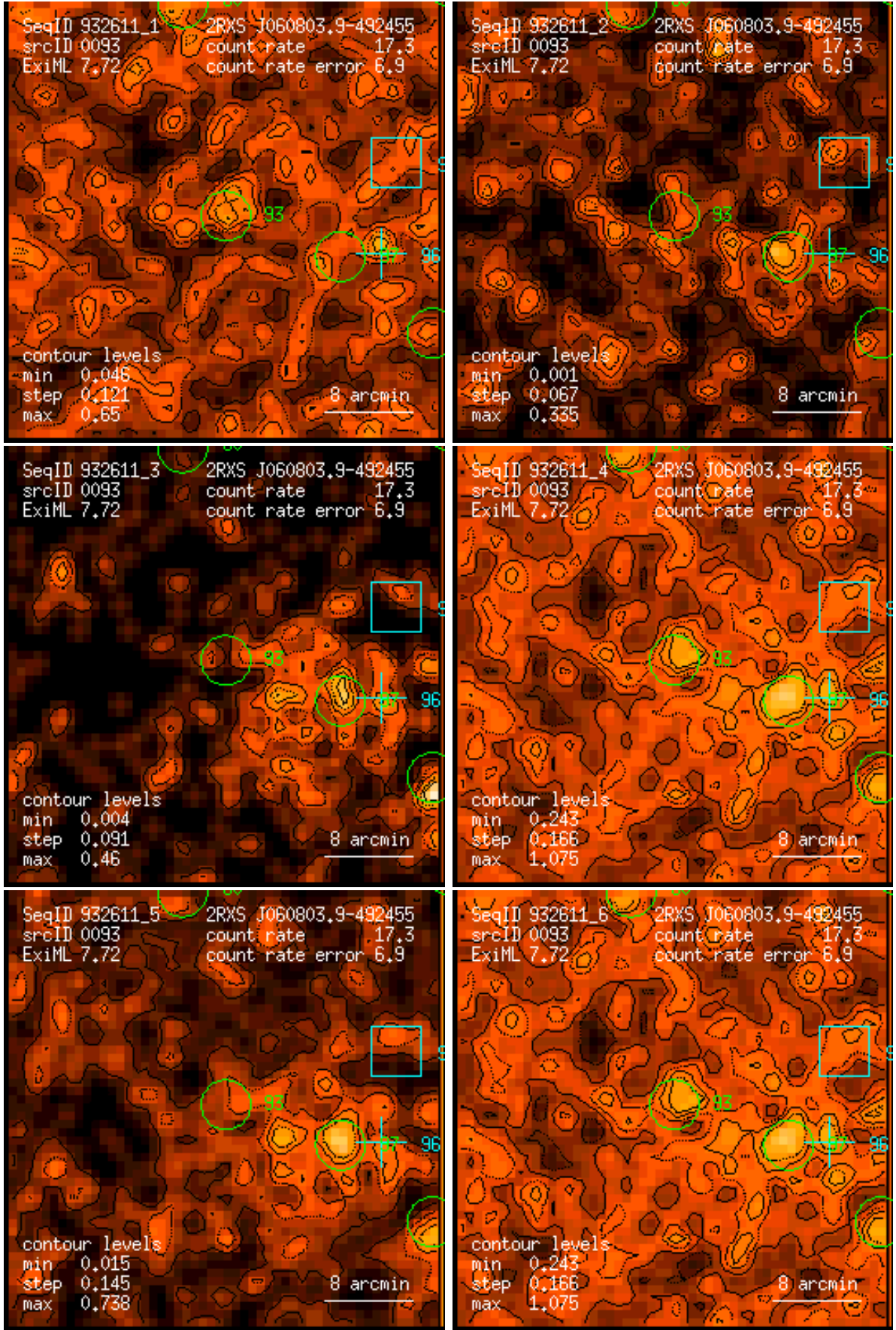
Figure 93: RASS 932611: detection 0093: band rate images, Gaussian filter: (1) PSPC channels 11 – 41, (2) 52 – 90, (3) 91 – 201, (4) 11 – 235, (5) 52 – 201, (6) 11 – 201. Broad band rates in counts/ks. Band rate contour levels in counts/ks/arcmin 2 .
