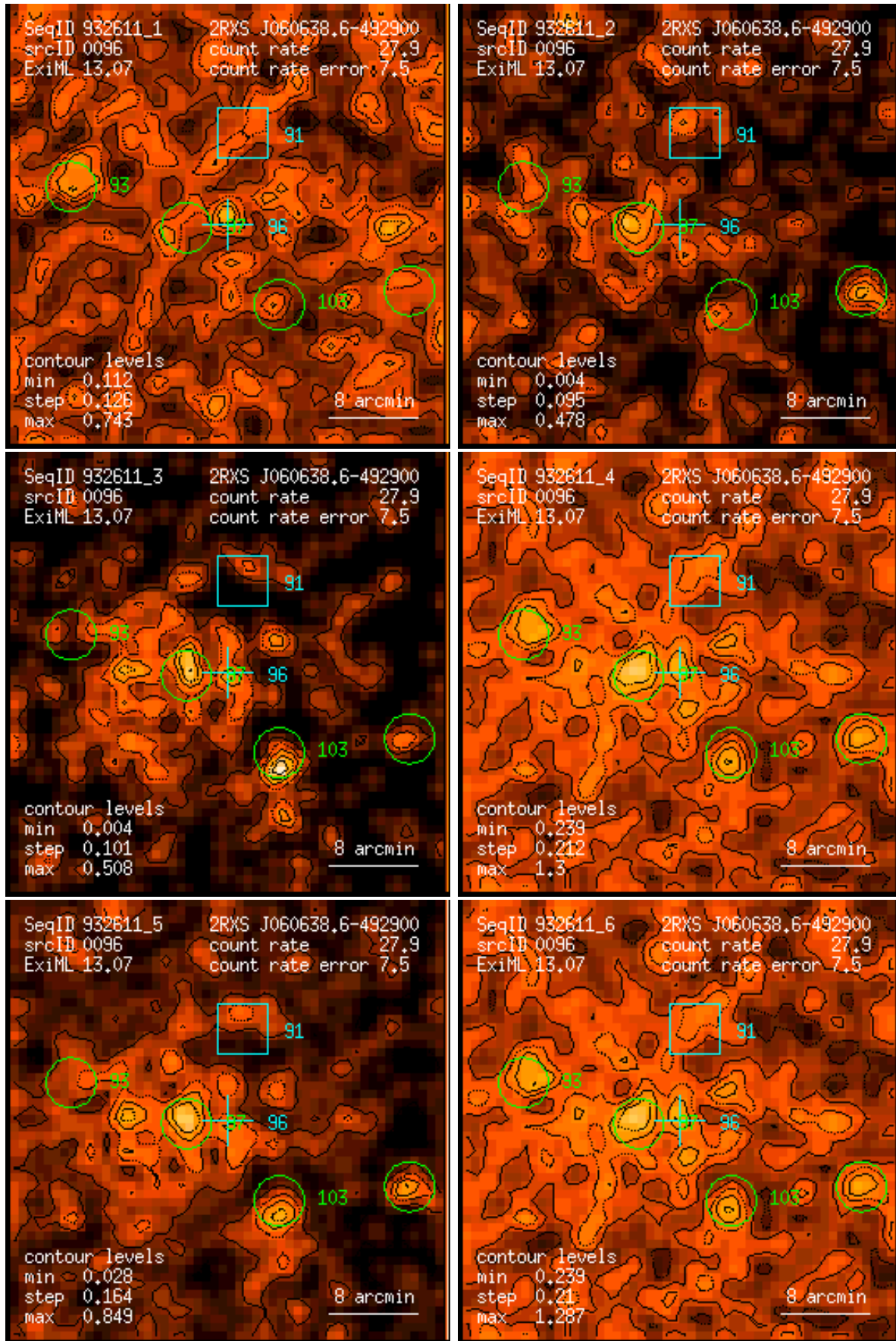
Figure 96: RASS 932611: detection 0096: band rate images, Gaussian filter: (1) PSPC channels 11 – 41, (2) 52 – 90, (3) 91 – 201, (4) 11 – 235, (5) 52 – 201, (6) 11 – 201. Broad band rates in counts/ks. Band rate contour levels in counts/ks/arcmin 2 .
