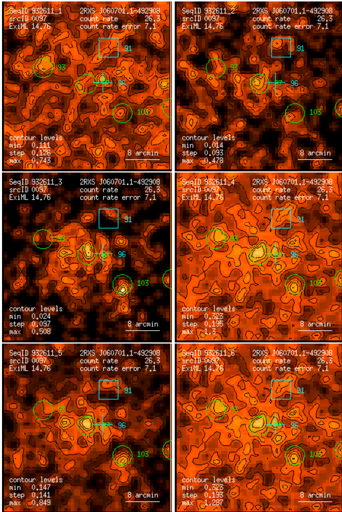
Figure 97: RASS 932611: detection 0097: band rate images, Gaussian filter: (1) PSPC channels 11 – 41, (2) 52 – 90, (3) 91 – 201, (4) 11 – 235, (5) 52 – 201, (6) 11 – 201. Broad band rates in counts/ks. Band rate contour levels in counts/ks/arcmin 2 .
