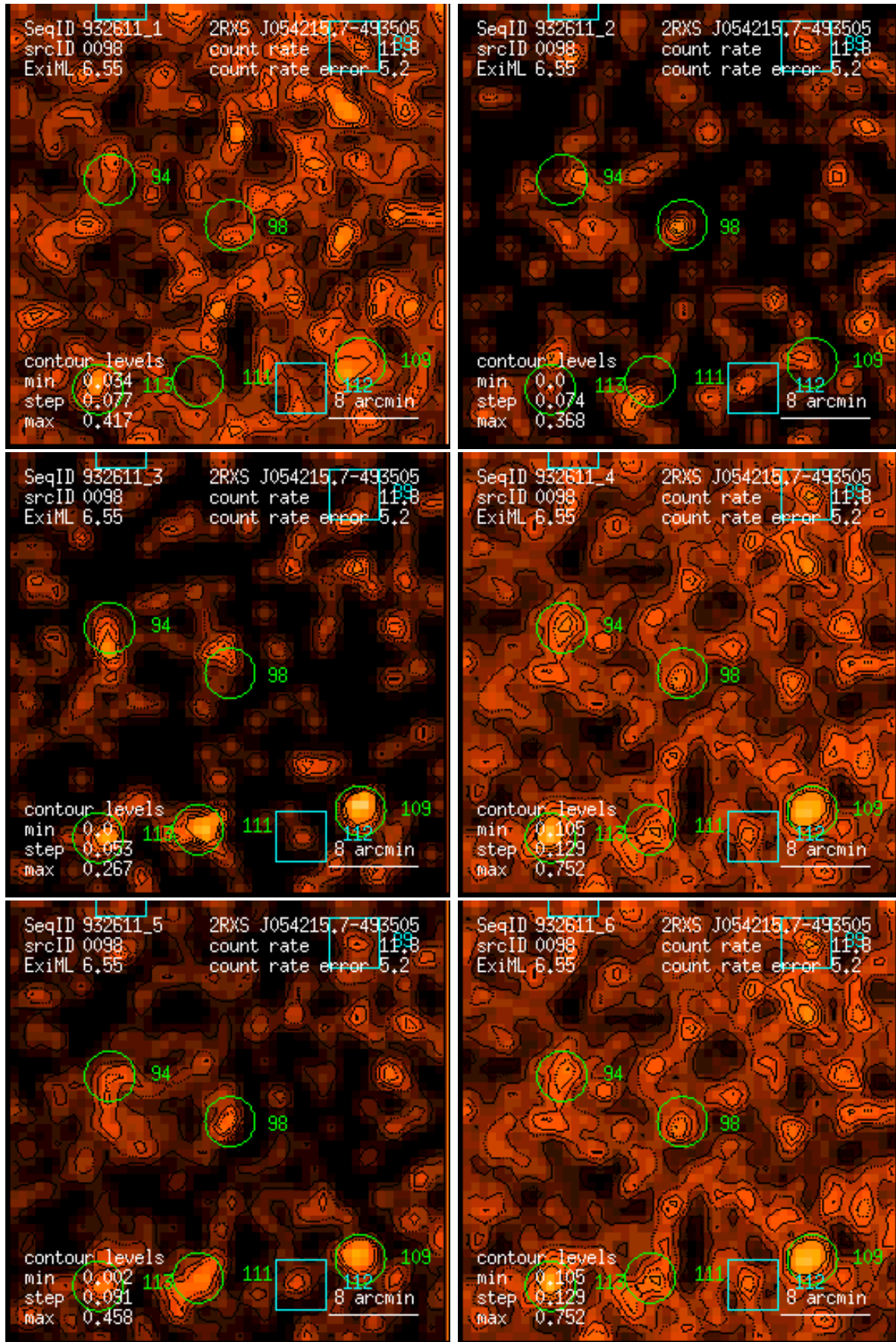
Figure 98: RASS 932611: detection 0098: band rate images, Gaussian filter: (1) PSPC channels 11 – 41, (2) 52 – 90, (3) 91 – 201, (4) 11 – 235, (5) 52 – 201, (6) 11 – 201. Broad band rates in counts/ks. Band rate contour levels in counts/ks/arcmin 2 .
