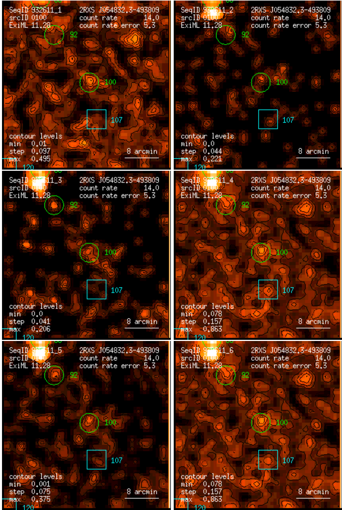
Figure 100: RASS 932611: detection 0100: band rate images, Gaussian filter: (1) PSPC channels 11 – 41, (2) 52 – 90, (3) 91 – 201, (4) 11 – 235, (5) 52 – 201, (6) 11 – 201. Broad band rates in counts/ks. Band rate contour levels in counts/ks/arcmin 2 .
