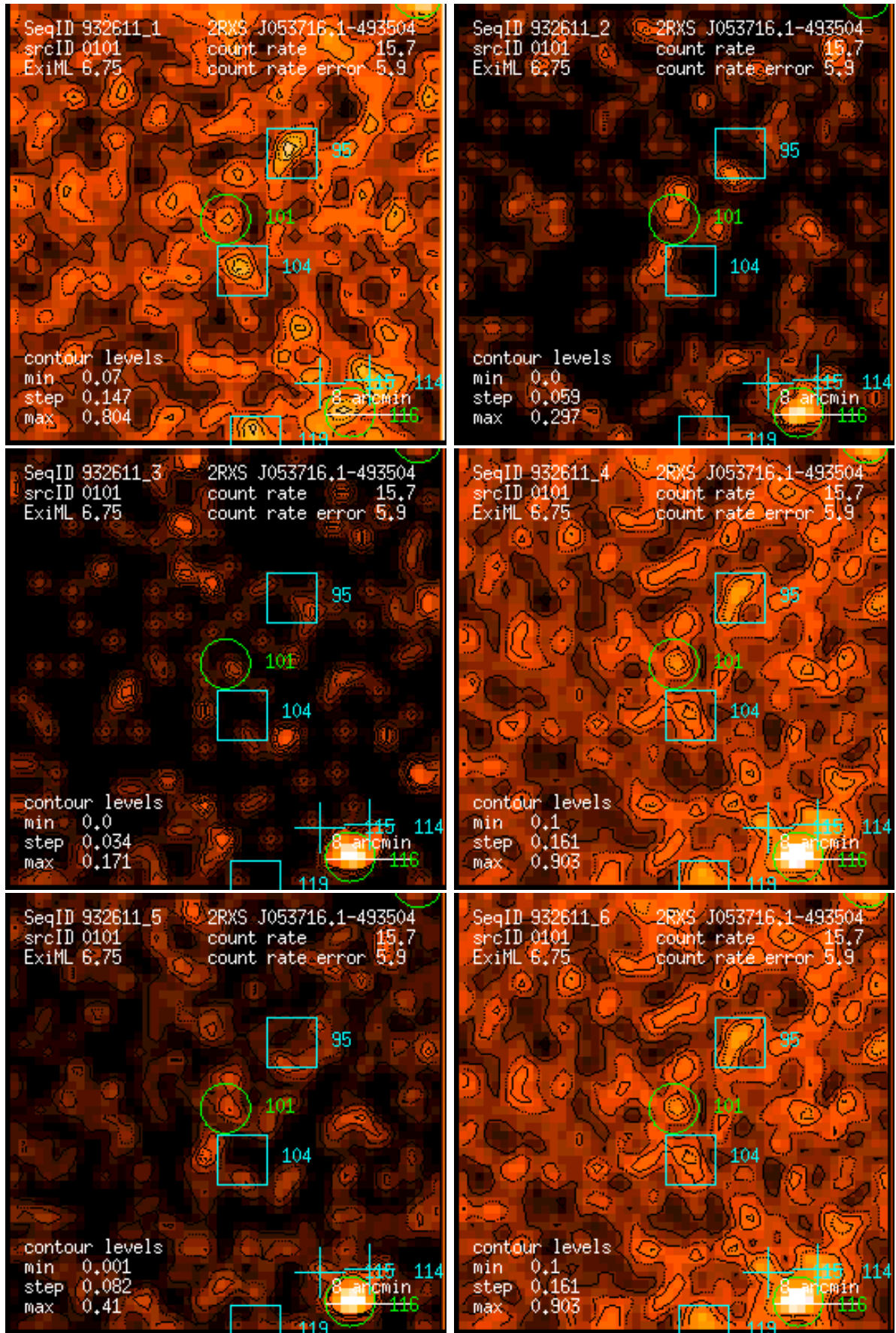
Figure 101: RASS 932611: detection 0101: band rate images, Gaussian filter: (1) PSPC channels 11 – 41, (2) 52 – 90, (3) 91 – 201, (4) 11 – 235, (5) 52 – 201, (6) 11 – 201. Broad band rates in counts/ks. Band rate contour levels in counts/ks/arcmin 2 .
