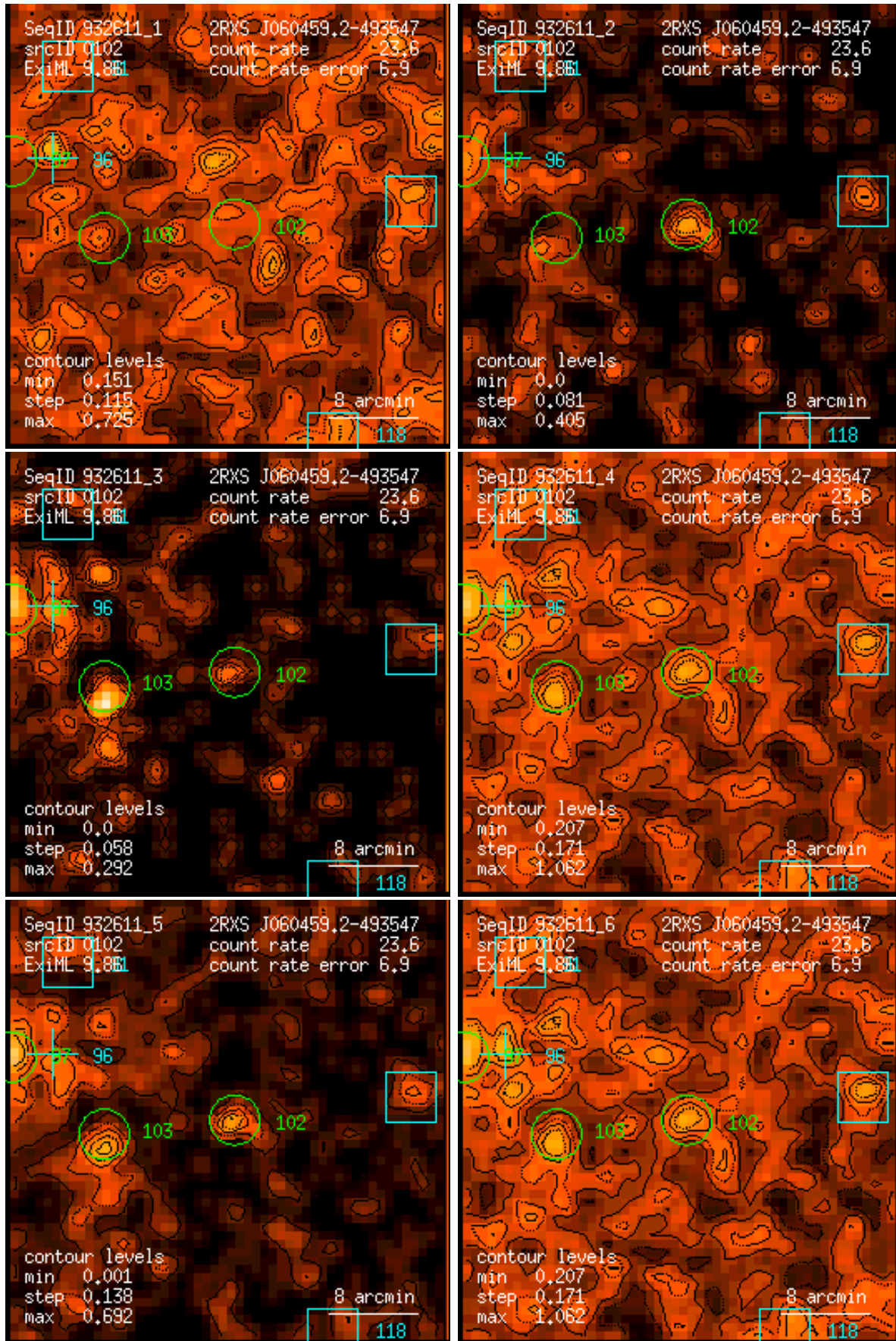
Figure 102: RASS 932611: detection 0102: band rate images, Gaussian filter: (1) PSPC channels 11 – 41, (2) 52 – 90, (3) 91 – 201, (4) 11 – 235, (5) 52 – 201, (6) 11 – 201. Broad band rates in counts/ks. Band rate contour levels in counts/ks/arcmin 2 .
