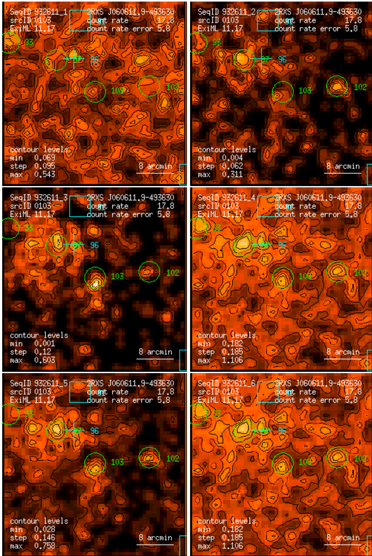
Figure 103: RASS 932611: detection 0103: band rate images, Gaussian filter: (1) PSPC channels 11 – 41, (2) 52 – 90, (3) 91 – 201, (4) 11 – 235, (5) 52 – 201, (6) 11 – 201. Broad band rates in counts/ks. Band rate contour levels in counts/ks/arcmin 2 .
