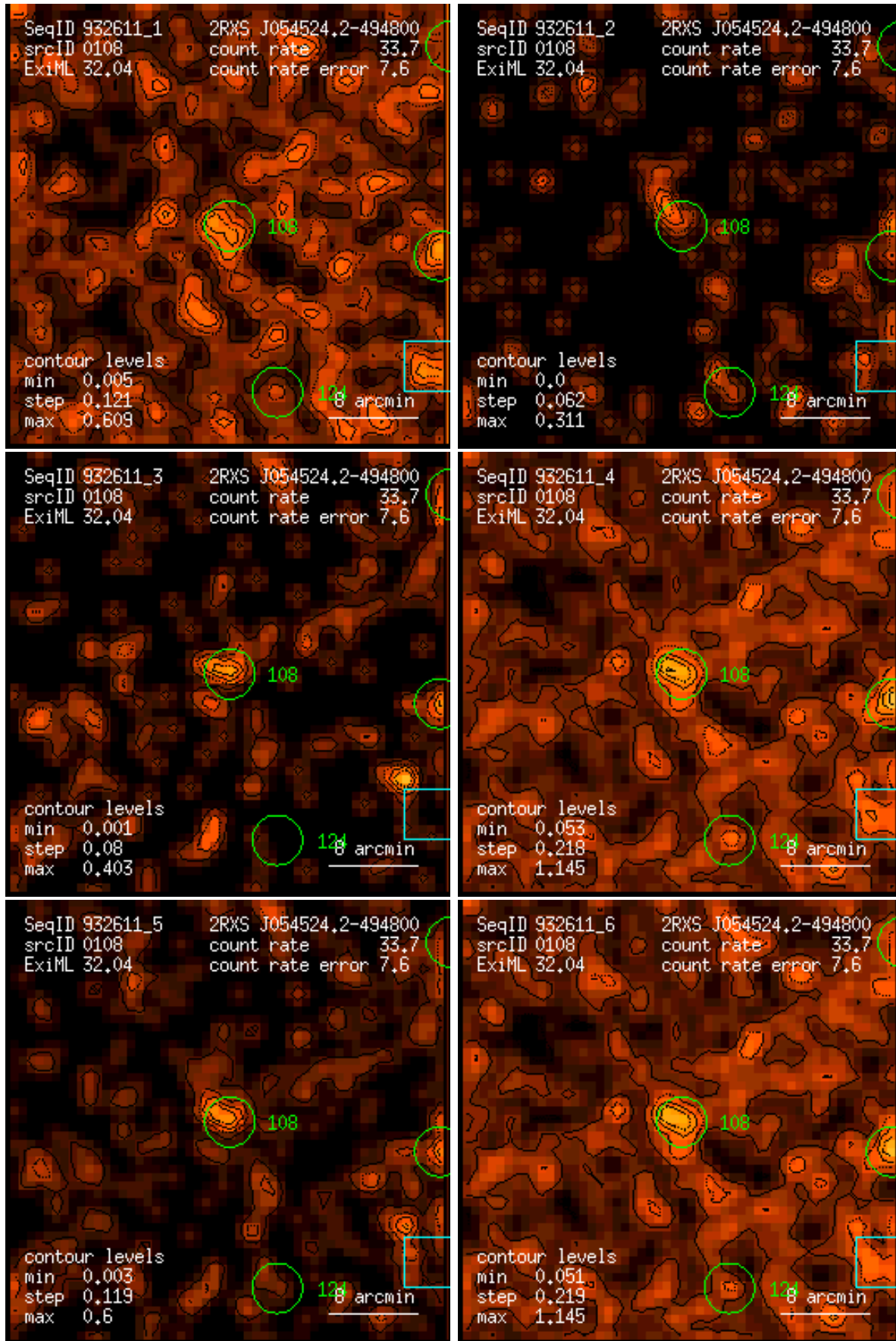
Figure 108: RASS 932611: detection 0108: band rate images, Gaussian filter: (1) PSPC channels 11 – 41, (2) 52 – 90, (3) 91 – 201, (4) 11 – 235, (5) 52 – 201, (6) 11 – 201. Broad band rates in counts/ks. Band rate contour levels in counts/ks/arcmin 2 .
