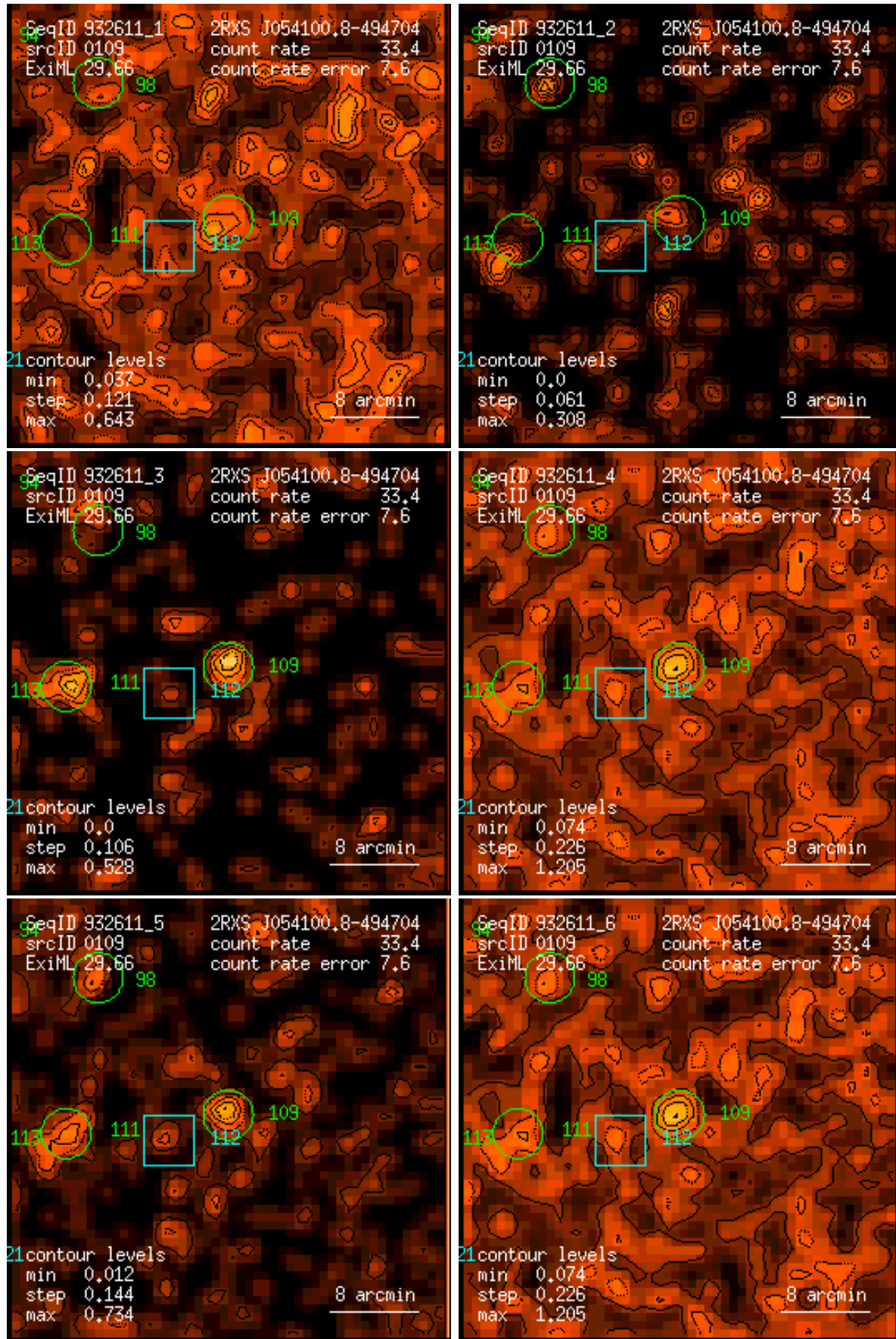
Figure 109: RASS 932611: detection 0109: band rate images, Gaussian filter: (1) PSPC channels 11 – 41, (2) 52 – 90, (3) 91 – 201, (4) 11 – 235, (5) 52 – 201, (6) 11 – 201. Broad band rates in counts/ks. Band rate contour levels in counts/ks/arcmin 2 .
