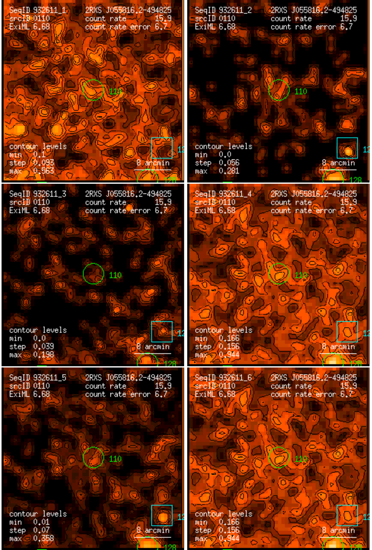
Figure 110: RASS 932611: detection 0110: band rate images, Gaussian filter: (1) PSPC channels 11 – 41, (2) 52 – 90, (3) 91 – 201, (4) 11 – 235, (5) 52 – 201, (6) 11 – 201. Broad band rates in counts/ks. Band rate contour levels in counts/ks/arcmin 2 .
