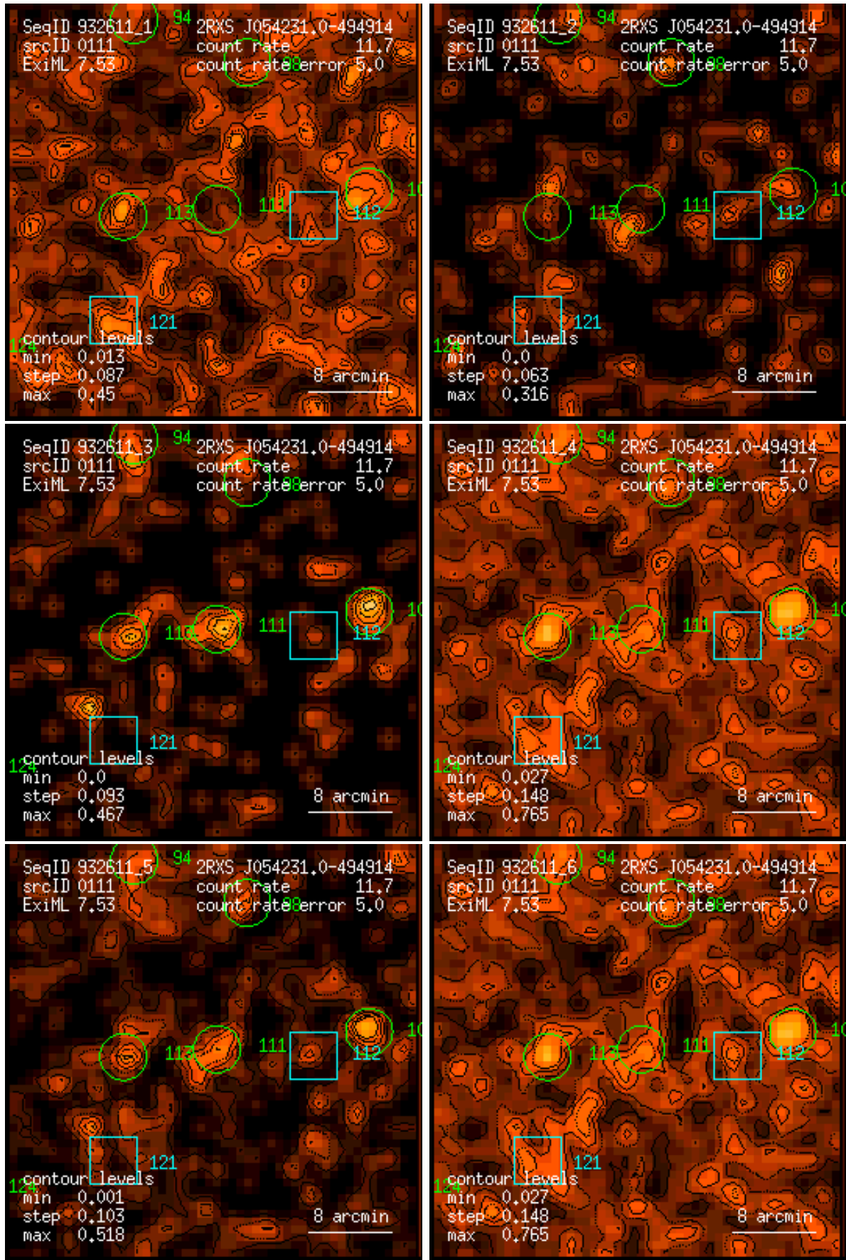
Figure 111: RASS 932611: detection 0111: band rate images, Gaussian filter: (1) PSPC channels 11 – 41, (2) 52 – 90, (3) 91 – 201, (4) 11 – 235, (5) 52 – 201, (6) 11 – 201. Broad band rates in counts/ks. Band rate contour levels in counts/ks/arcmin 2 .
