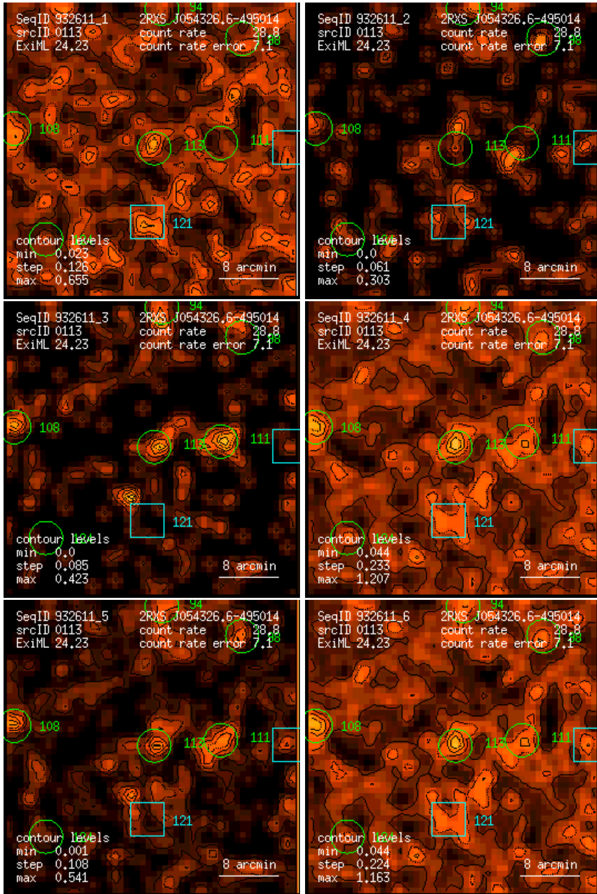
Figure 113: RASS 932611: detection 0113: band rate images, Gaussian filter: (1) PSPC channels 11 – 41, (2) 52 – 90, (3) 91 – 201, (4) 11 – 235, (5) 52 – 201, (6) 11 – 201. Broad band rates in counts/ks. Band rate contour levels in counts/ks/arcmin 2 .
