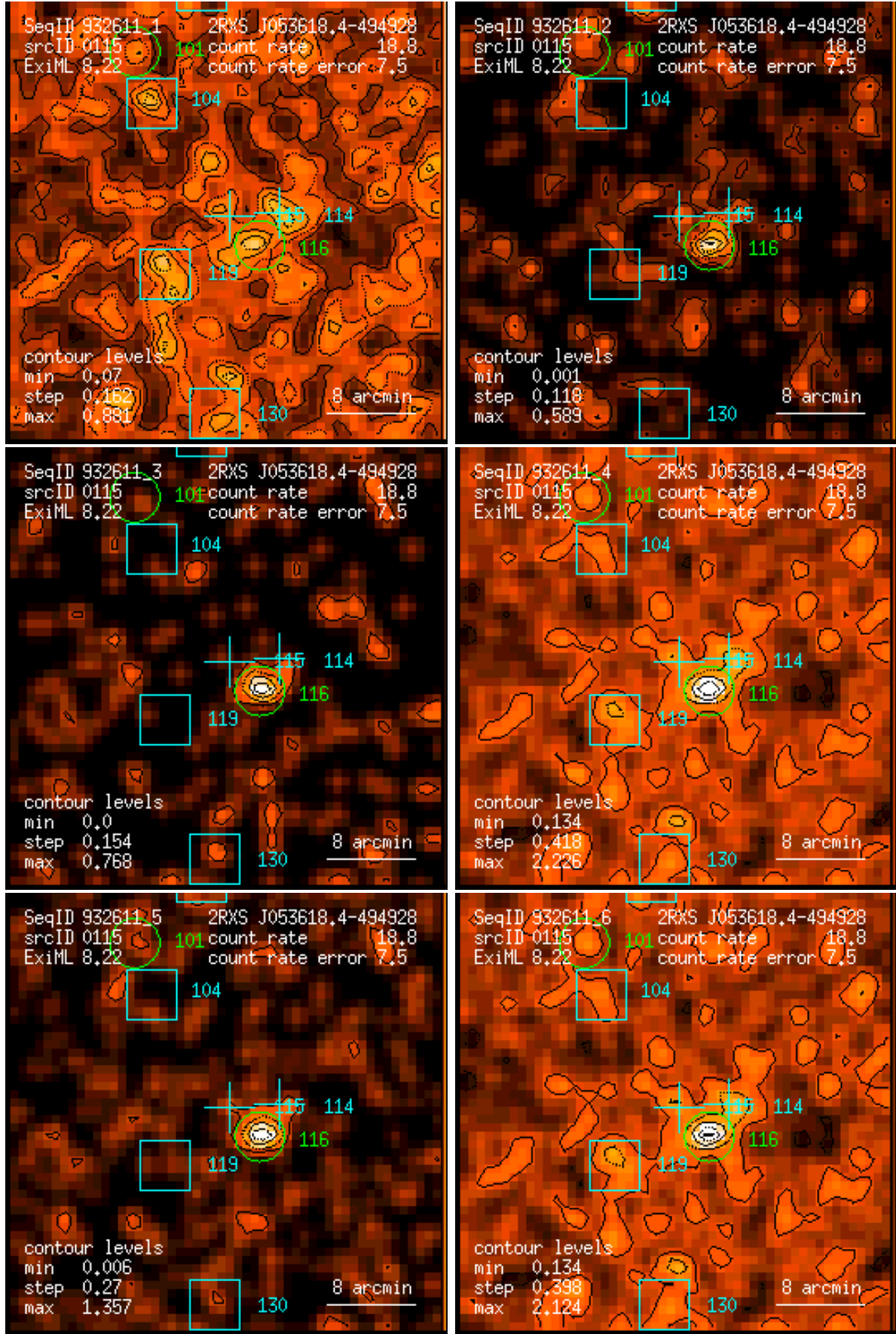
Figure 115: RASS 932611: detection 0115: band rate images, Gaussian filter: (1) PSPC channels 11 – 41, (2) 52 – 90, (3) 91 – 201, (4) 11 – 235, (5) 52 – 201, (6) 11 – 201. Broad band rates in counts/ks. Band rate contour levels in counts/ks/arcmin 2 .
