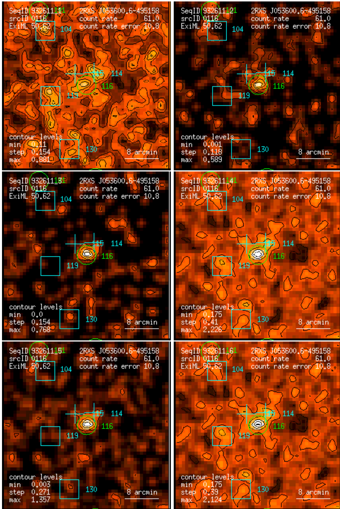
Figure 116: RASS 932611: detection 0116: band rate images, Gaussian filter: (1) PSPC channels 11 – 41, (2) 52 – 90, (3) 91 – 201, (4) 11 – 235, (5) 52 – 201, (6) 11 – 201. Broad band rates in counts/ks. Band rate contour levels in counts/ks/arcmin 2 .
