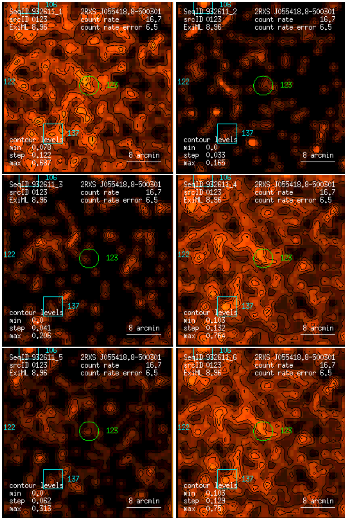
Figure 123: RASS 932611: detection 0123: band rate images, Gaussian filter: (1) PSPC channels 11 – 41, (2) 52 – 90, (3) 91 – 201, (4) 11 – 235, (5) 52 – 201, (6) 11 – 201. Broad band rates in counts/ks. Band rate contour levels in counts/ks/arcmin 2 .
