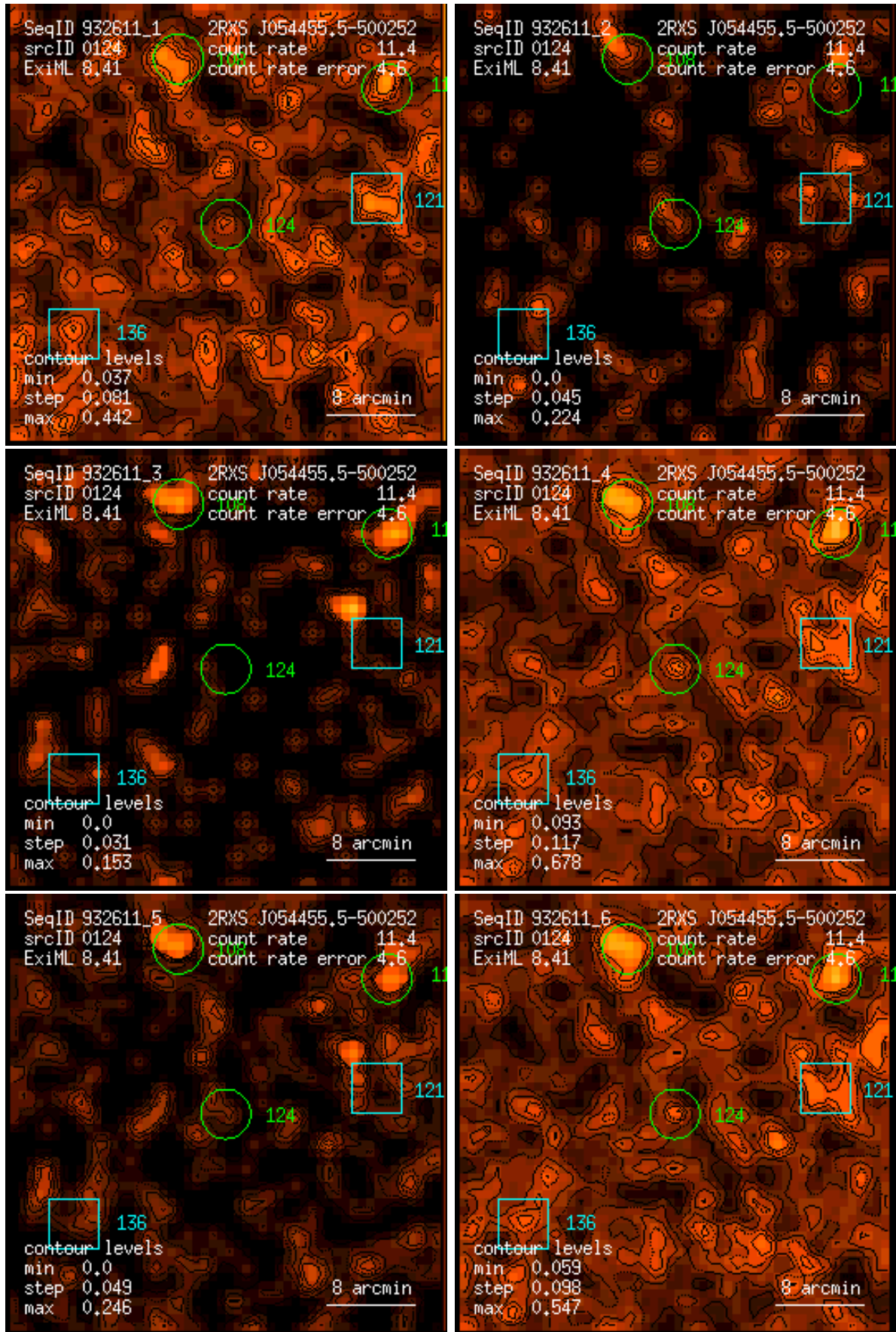
Figure 124: RASS 932611: detection 0124: band rate images, Gaussian filter: (1) PSPC channels 11 – 41, (2) 52 – 90, (3) 91 – 201, (4) 11 – 235, (5) 52 – 201, (6) 11 – 201. Broad band rates in counts/ks. Band rate contour levels in counts/ks/arcmin 2 .
