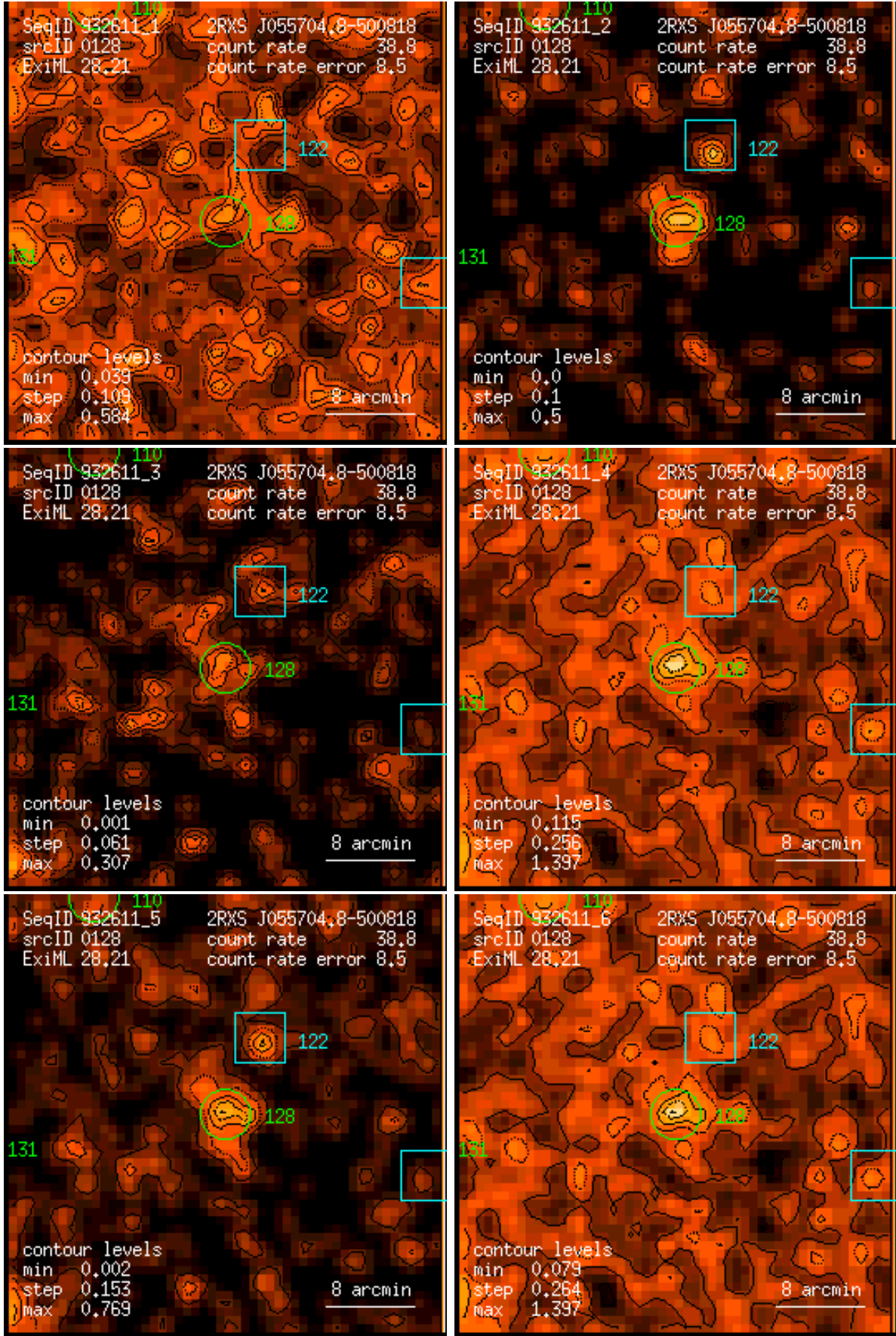
Figure 128: RASS 932611: detection 0128: band rate images, Gaussian filter: (1) PSPC channels 11 – 41, (2) 52 – 90, (3) 91 – 201, (4) 11 – 235, (5) 52 – 201, (6) 11 – 201. Broad band rates in counts/ks. Band rate contour levels in counts/ks/arcmin 2 .
