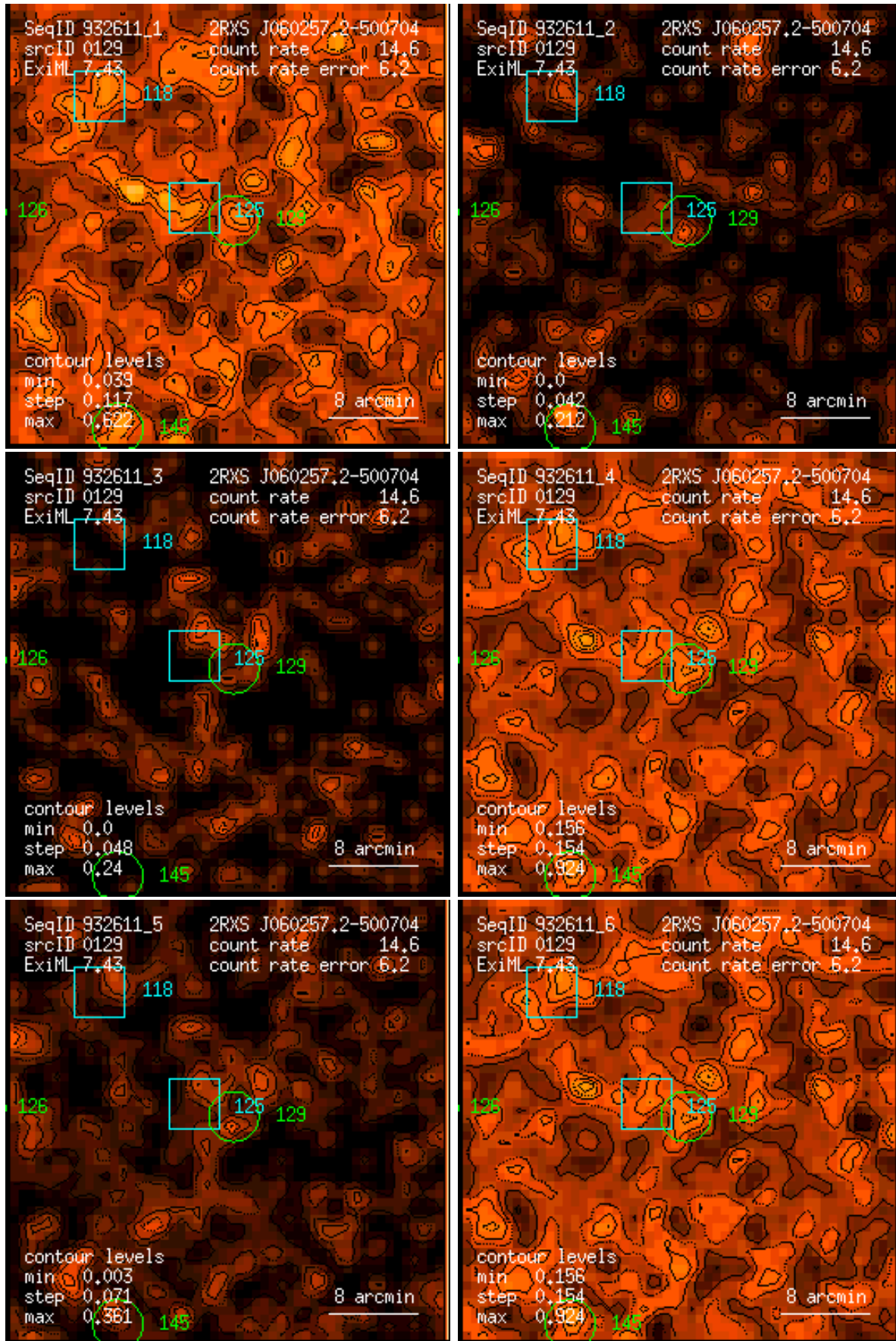
Figure 129: RASS 932611: detection 0129: band rate images, Gaussian filter: (1) PSPC channels 11 – 41, (2) 52 – 90, (3) 91 – 201, (4) 11 – 235, (5) 52 – 201, (6) 11 – 201. Broad band rates in counts/ks. Band rate contour levels in counts/ks/arcmin 2 .
