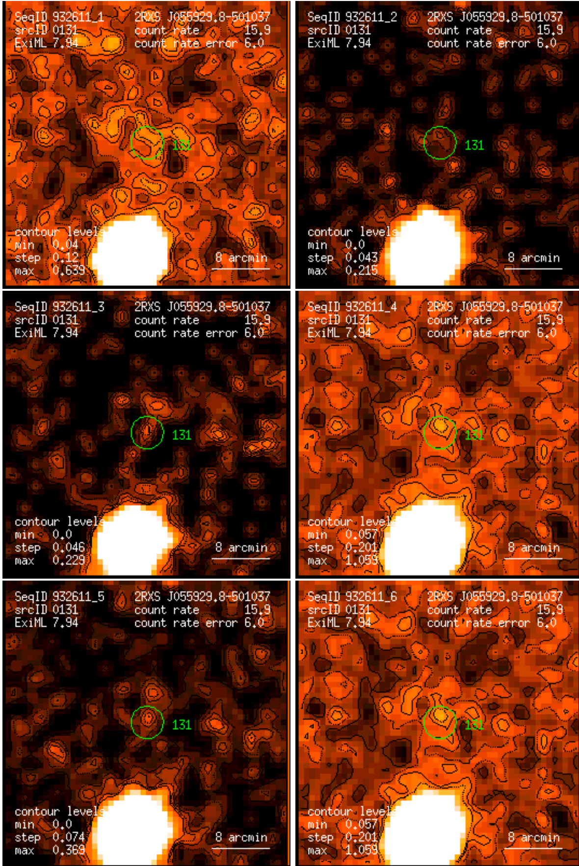
Figure 131: RASS 932611: detection 0131: band rate images, Gaussian filter: (1) PSPC channels 11 – 41, (2) 52 – 90, (3) 91 – 201, (4) 11 – 235, (5) 52 – 201, (6) 11 – 201. Broad band rates in counts/ks. Band rate contour levels in counts/ks/arcmin 2 .
