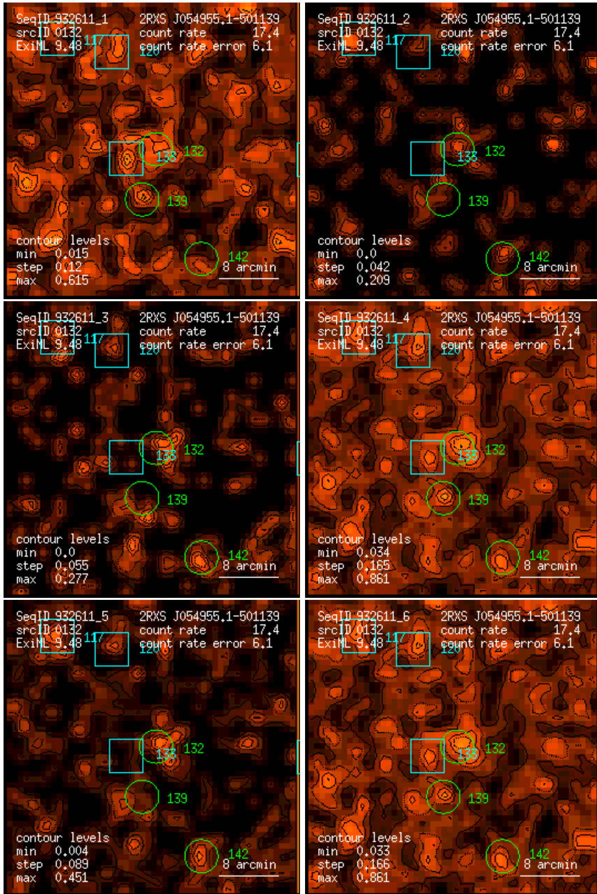
Figure 132: RASS 932611: detection 0132: band rate images, Gaussian filter: (1) PSPC channels 11 – 41, (2) 52 – 90, (3) 91 – 201, (4) 11 – 235, (5) 52 – 201, (6) 11 – 201. Broad band rates in counts/ks. Band rate contour levels in counts/ks/arcmin 2 .
