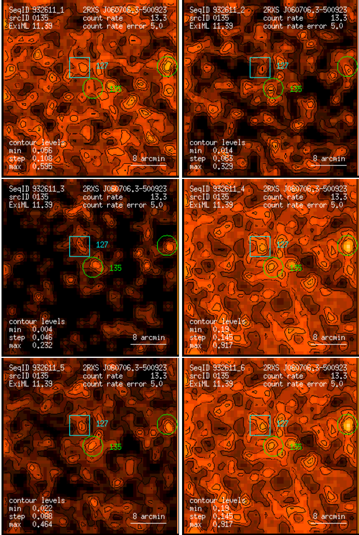
Figure 135: RASS 932611: detection 0135: band rate images, Gaussian filter: (1) PSPC channels 11 – 41, (2) 52 – 90, (3) 91 – 201, (4) 11 – 235, (5) 52 – 201, (6) 11 – 201. Broad band rates in counts/ks. Band rate contour levels in counts/ks/arcmin 2 .
