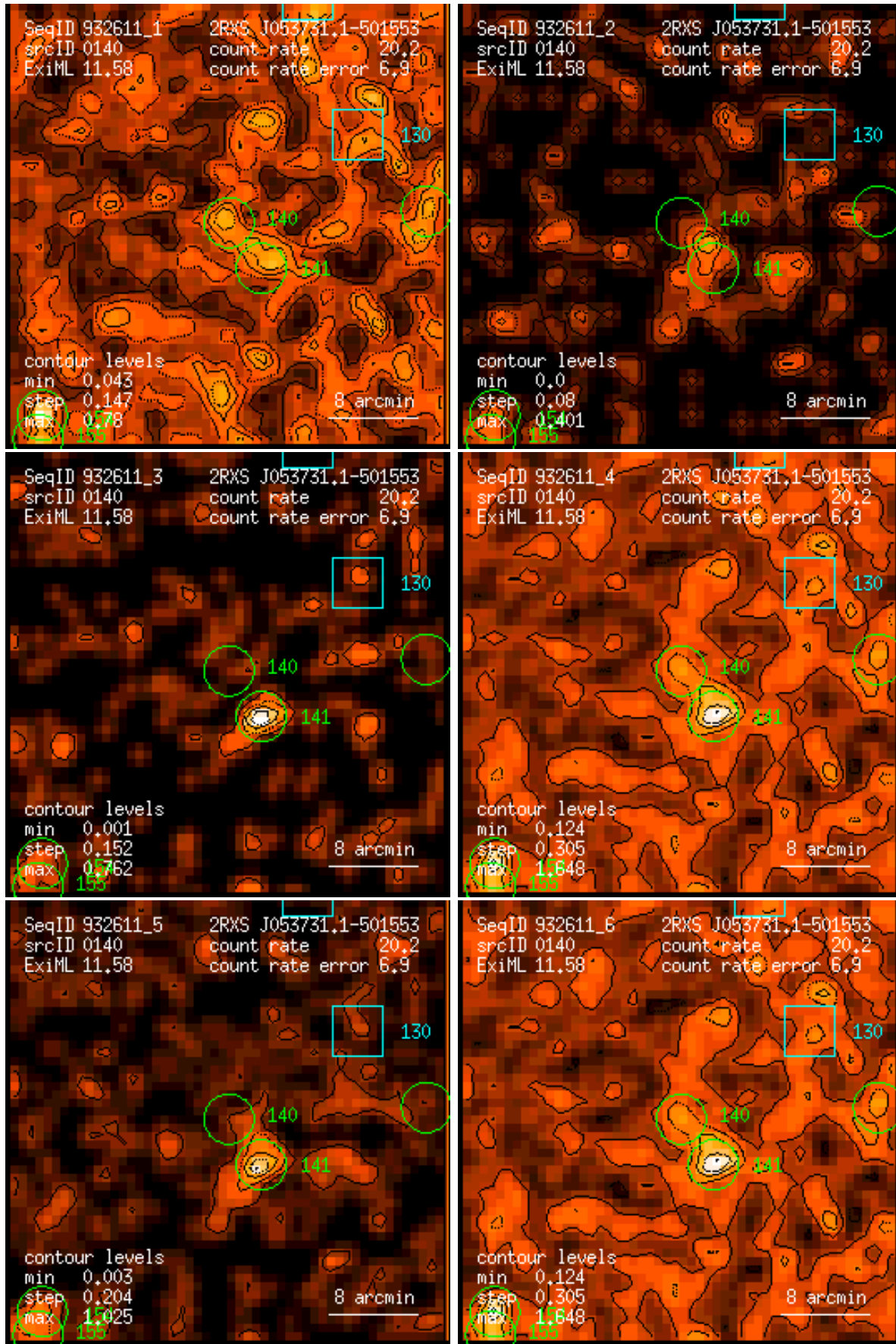
Figure 140: RASS 932611: detection 0140: band rate images, Gaussian filter: (1) PSPC channels 11 – 41, (2) 52 – 90, (3) 91 – 201, (4) 11 – 235, (5) 52 – 201, (6) 11 – 201. Broad band rates in counts/ks. Band rate contour levels in counts/ks/arcmin 2 .
