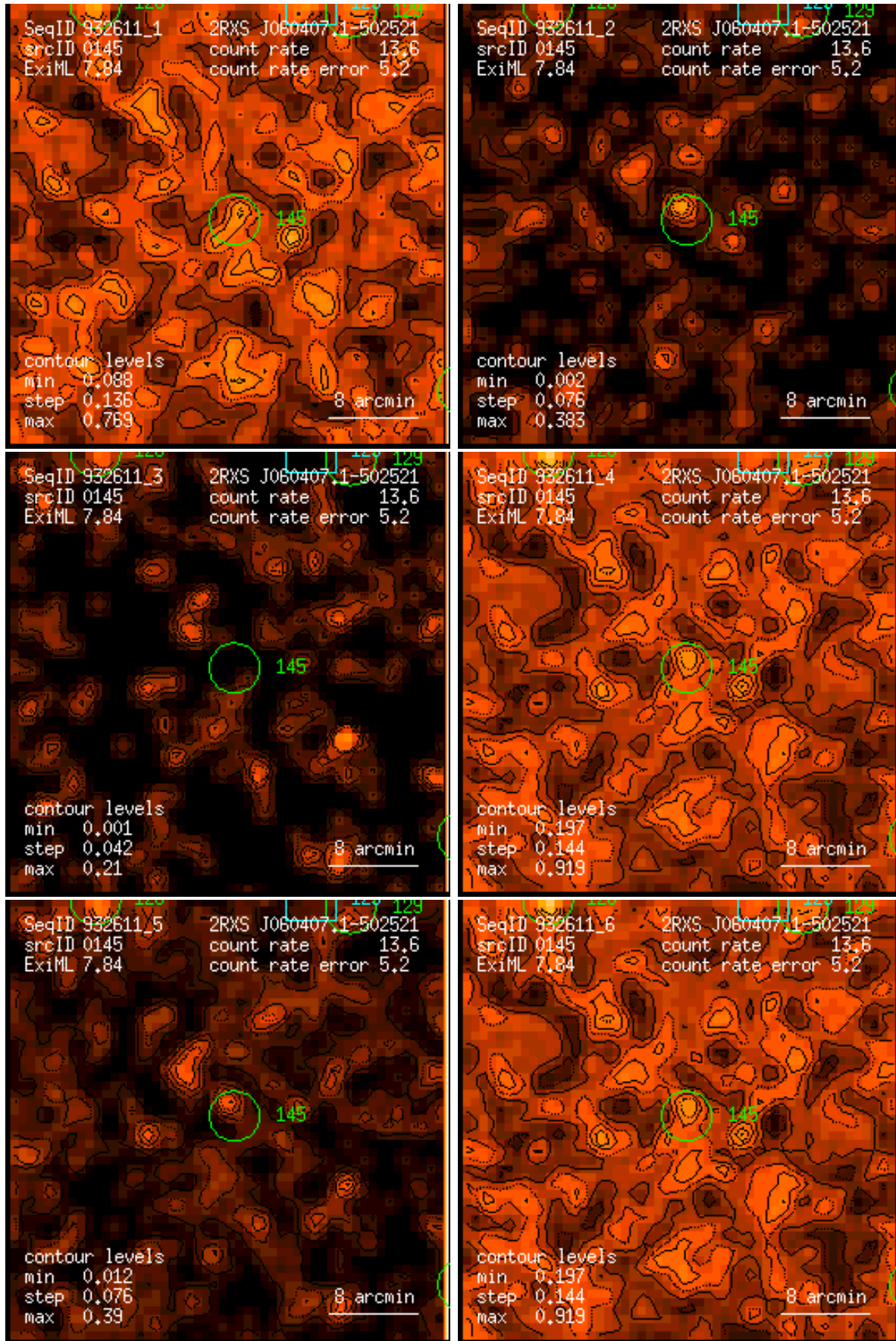
Figure 145: RASS 932611: detection 0145: band rate images, Gaussian filter: (1) PSPC channels 11 – 41, (2) 52 – 90, (3) 91 – 201, (4) 11 – 235, (5) 52 – 201, (6) 11 – 201. Broad band rates in counts/ks. Band rate contour levels in counts/ks/arcmin 2 .
