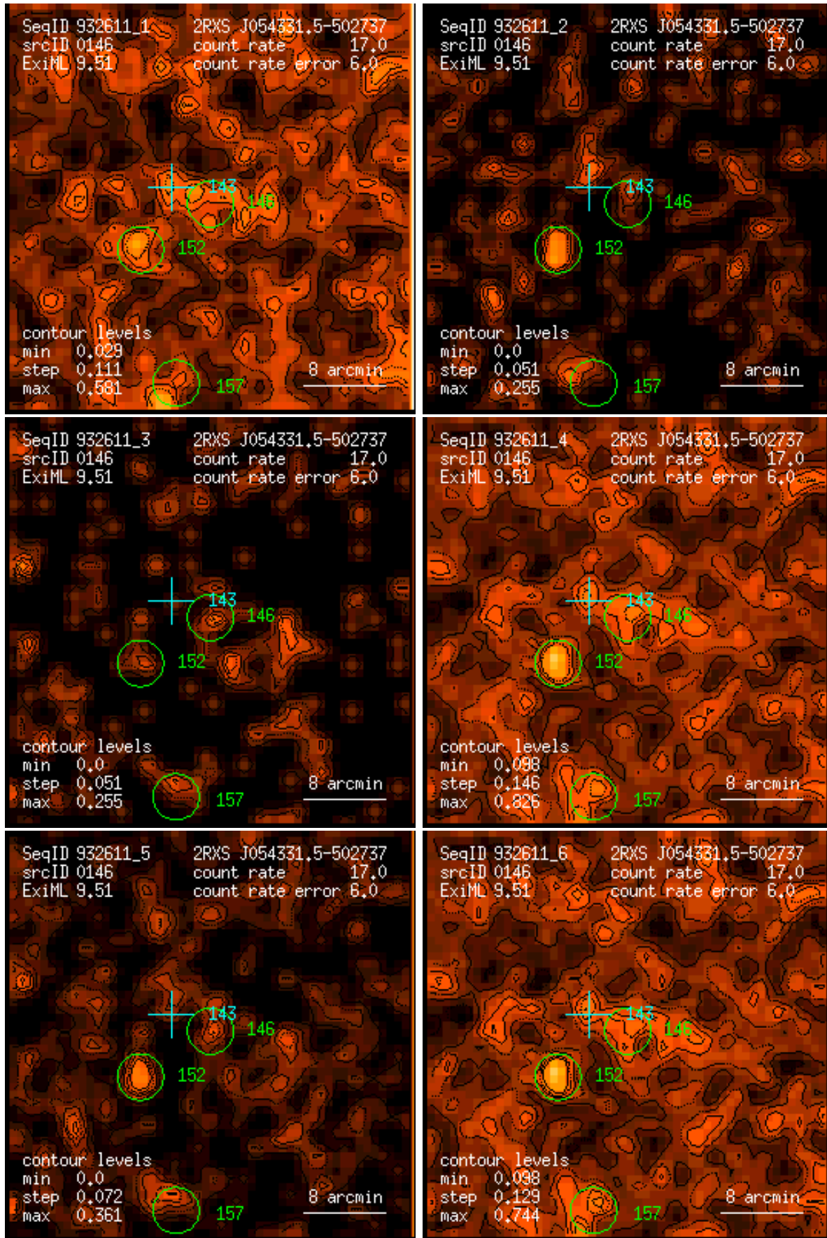
Figure 146: RASS 932611: detection 0146: band rate images, Gaussian filter: (1) PSPC channels 11 – 41, (2) 52 – 90, (3) 91 – 201, (4) 11 – 235, (5) 52 – 201, (6) 11 – 201. Broad band rates in counts/ks. Band rate contour levels in counts/ks/arcmin 2 .
