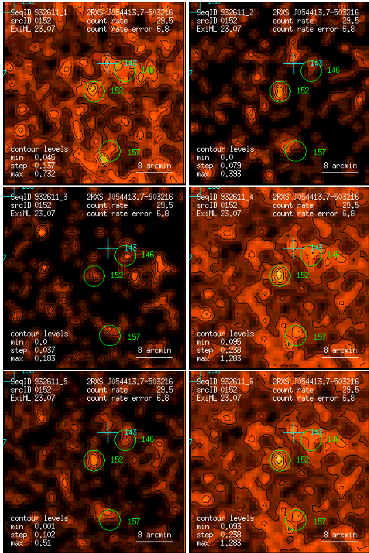
Figure 152: RASS 932611: detection 0152: band rate images, Gaussian filter: (1) PSPC channels 11 – 41, (2) 52 – 90, (3) 91 – 201, (4) 11 – 235, (5) 52 – 201, (6) 11 – 201. Broad band rates in counts/ks. Band rate contour levels in counts/ks/arcmin 2 .
