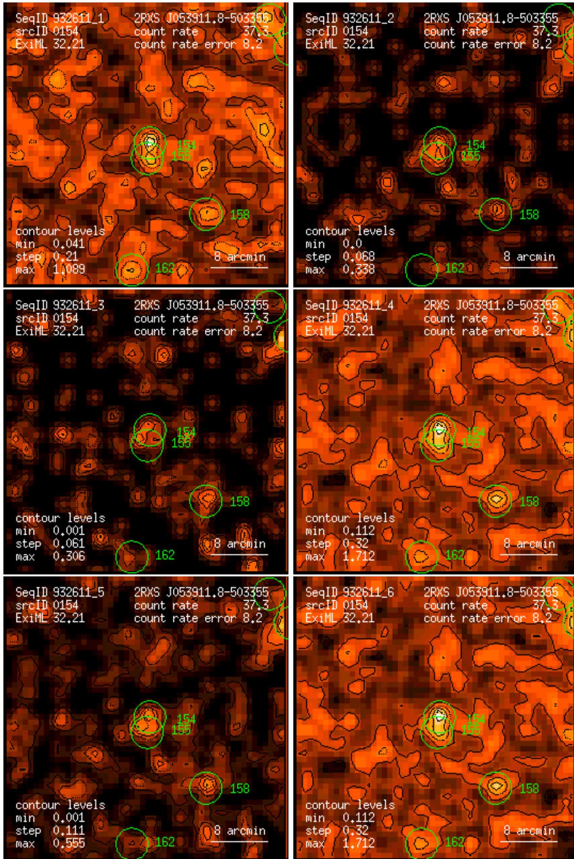
Figure 154: RASS 932611: detection 0154: band rate images, Gaussian filter: (1) PSPC channels 11 – 41, (2) 52 – 90, (3) 91 – 201, (4) 11 – 235, (5) 52 – 201, (6) 11 – 201. Broad band rates in counts/ks. Band rate contour levels in counts/ks/arcmin 2 .
