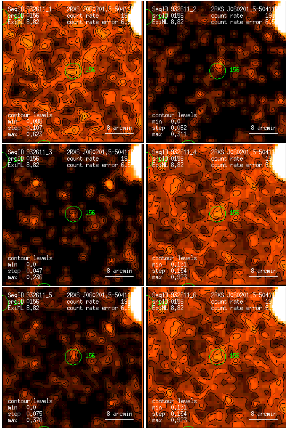
Figure 156: RASS 932611: detection 0156: band rate images, Gaussian filter: (1) PSPC channels 11 – 41, (2) 52 – 90, (3) 91 – 201, (4) 11 – 235, (5) 52 – 201, (6) 11 – 201. Broad band rates in counts/ks. Band rate contour levels in counts/ks/arcmin 2 .
