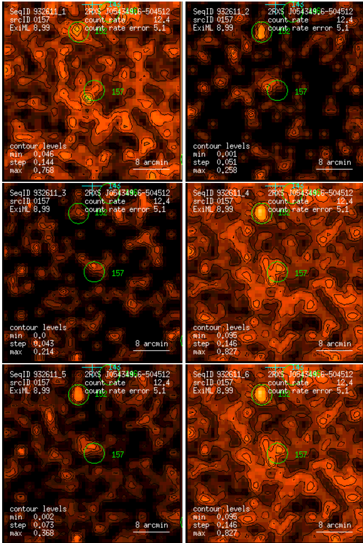
Figure 157: RASS 932611: detection 0157: band rate images, Gaussian filter: (1) PSPC channels 11 – 41, (2) 52 – 90, (3) 91 – 201, (4) 11 – 235, (5) 52 – 201, (6) 11 – 201. Broad band rates in counts/ks. Band rate contour levels in counts/ks/arcmin 2 .
