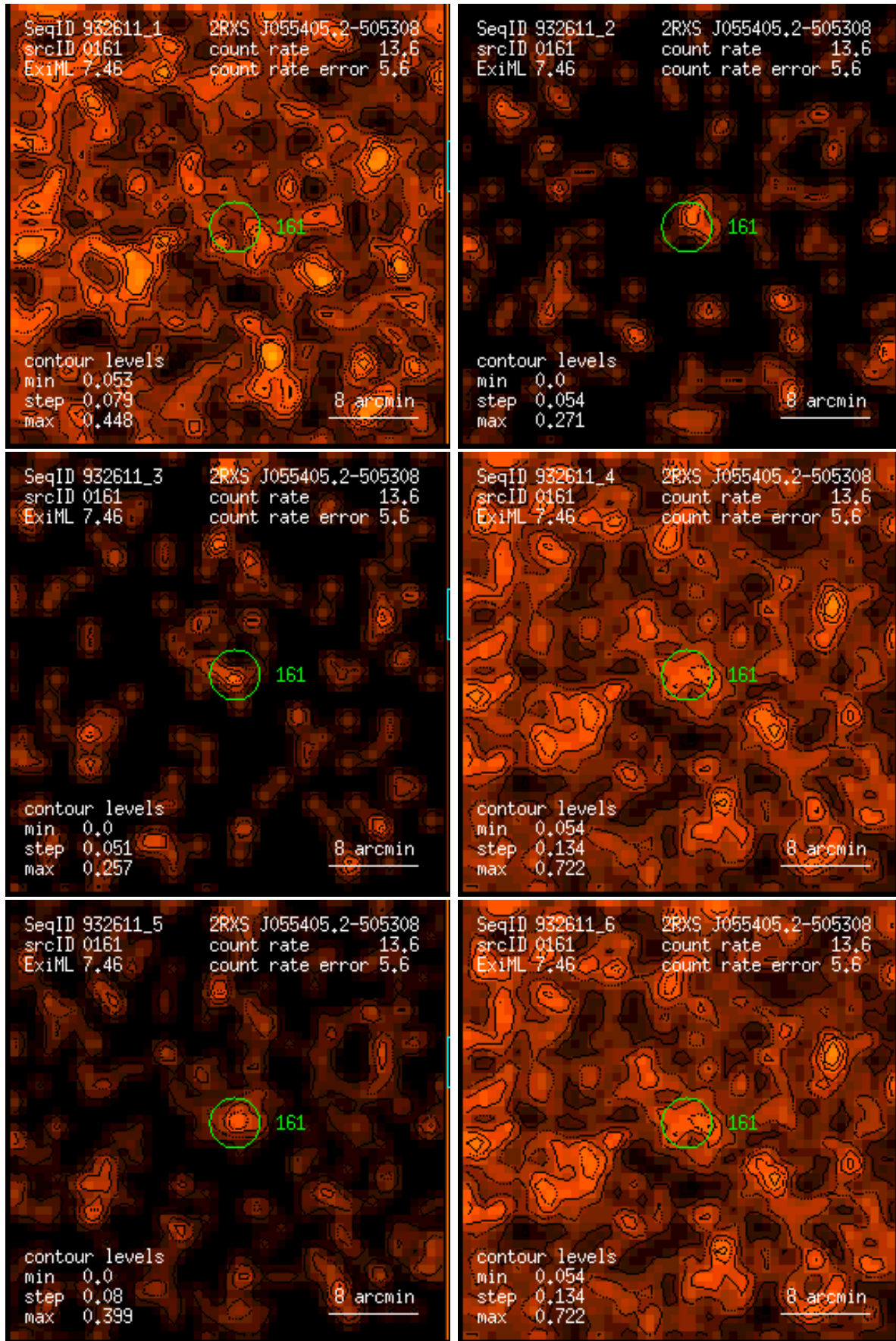
Figure 161: RASS 932611: detection 0161: band rate images, Gaussian filter: (1) PSPC channels 11 – 41, (2) 52 – 90, (3) 91 – 201, (4) 11 – 235, (5) 52 – 201, (6) 11 – 201. Broad band rates in counts/ks. Band rate contour levels in counts/ks/arcmin 2 .
