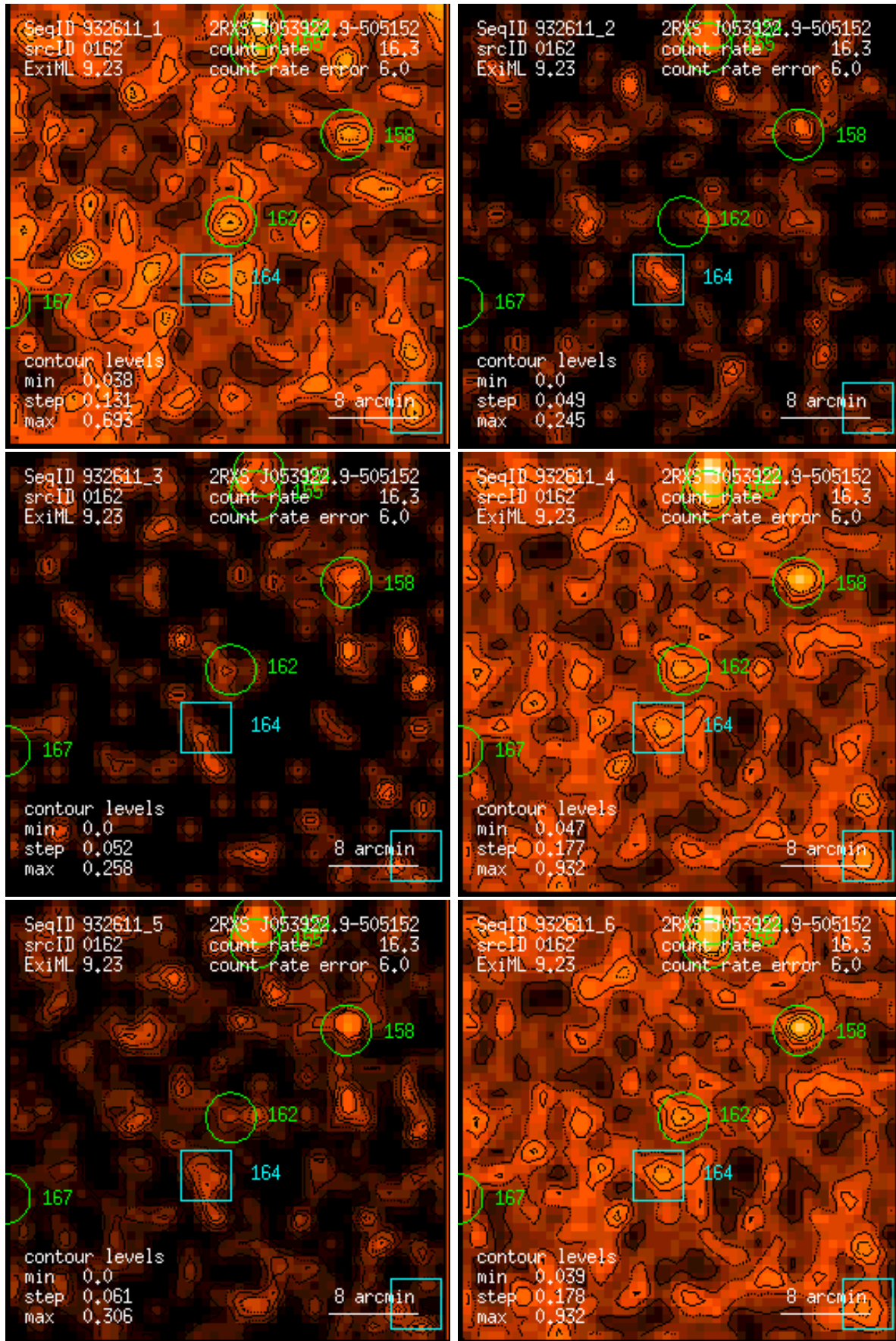
Figure 162: RASS 932611: detection 0162: band rate images, Gaussian filter: (1) PSPC channels 11 – 41, (2) 52 – 90, (3) 91 – 201, (4) 11 – 235, (5) 52 – 201, (6) 11 – 201. Broad band rates in counts/ks. Band rate contour levels in counts/ks/arcmin 2 .
