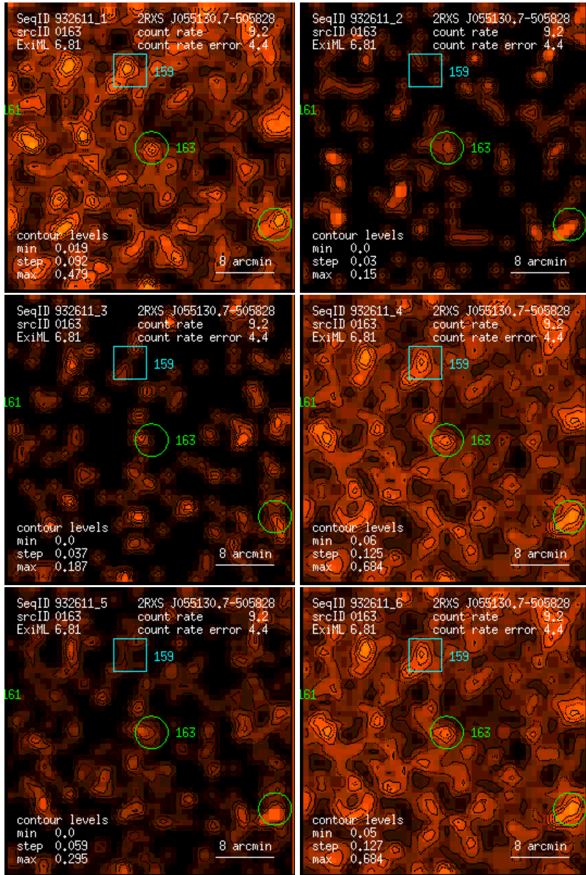
Figure 163: RASS 932611: detection 0163: band rate images, Gaussian filter: (1) PSPC channels 11 – 41, (2) 52 – 90, (3) 91 – 201, (4) 11 – 235, (5) 52 – 201, (6) 11 – 201. Broad band rates in counts/ks. Band rate contour levels in counts/ks/arcmin 2 .
