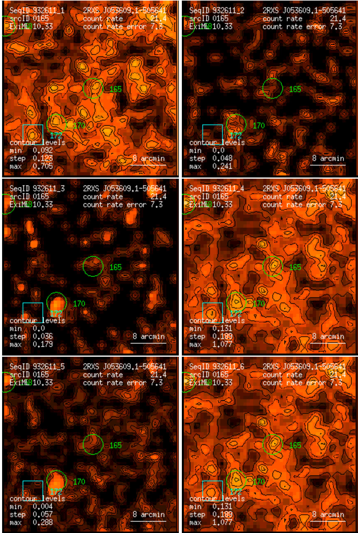
Figure 165: RASS 932611: detection 0165: band rate images, Gaussian filter: (1) PSPC channels 11 – 41, (2) 52 – 90, (3) 91 – 201, (4) 11 – 235, (5) 52 – 201, (6) 11 – 201. Broad band rates in counts/ks. Band rate contour levels in counts/ks/arcmin 2 .
