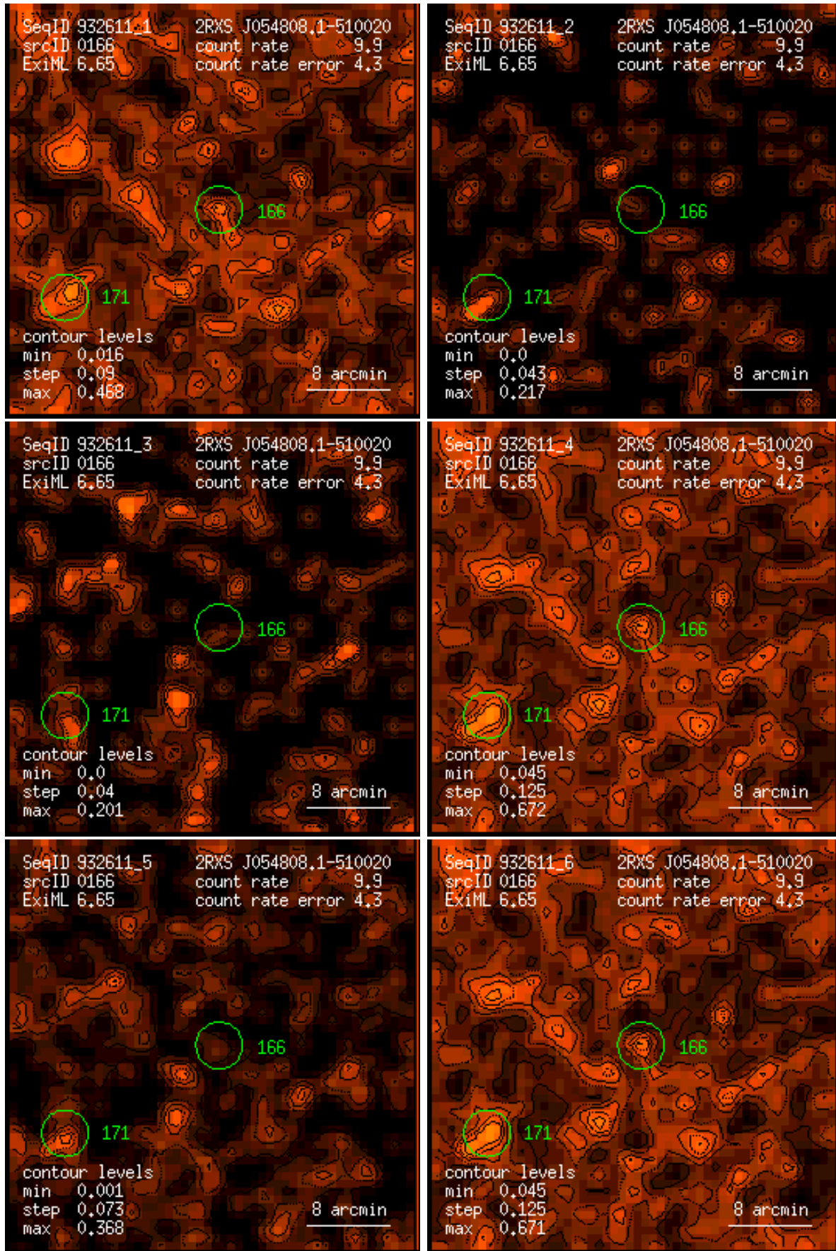
Figure 166: RASS 932611: detection 0166: band rate images, Gaussian filter: (1) PSPC channels 11 – 41, (2) 52 – 90, (3) 91 – 201, (4) 11 – 235, (5) 52 – 201, (6) 11 – 201. Broad band rates in counts/ks. Band rate contour levels in counts/ks/arcmin 2 .
