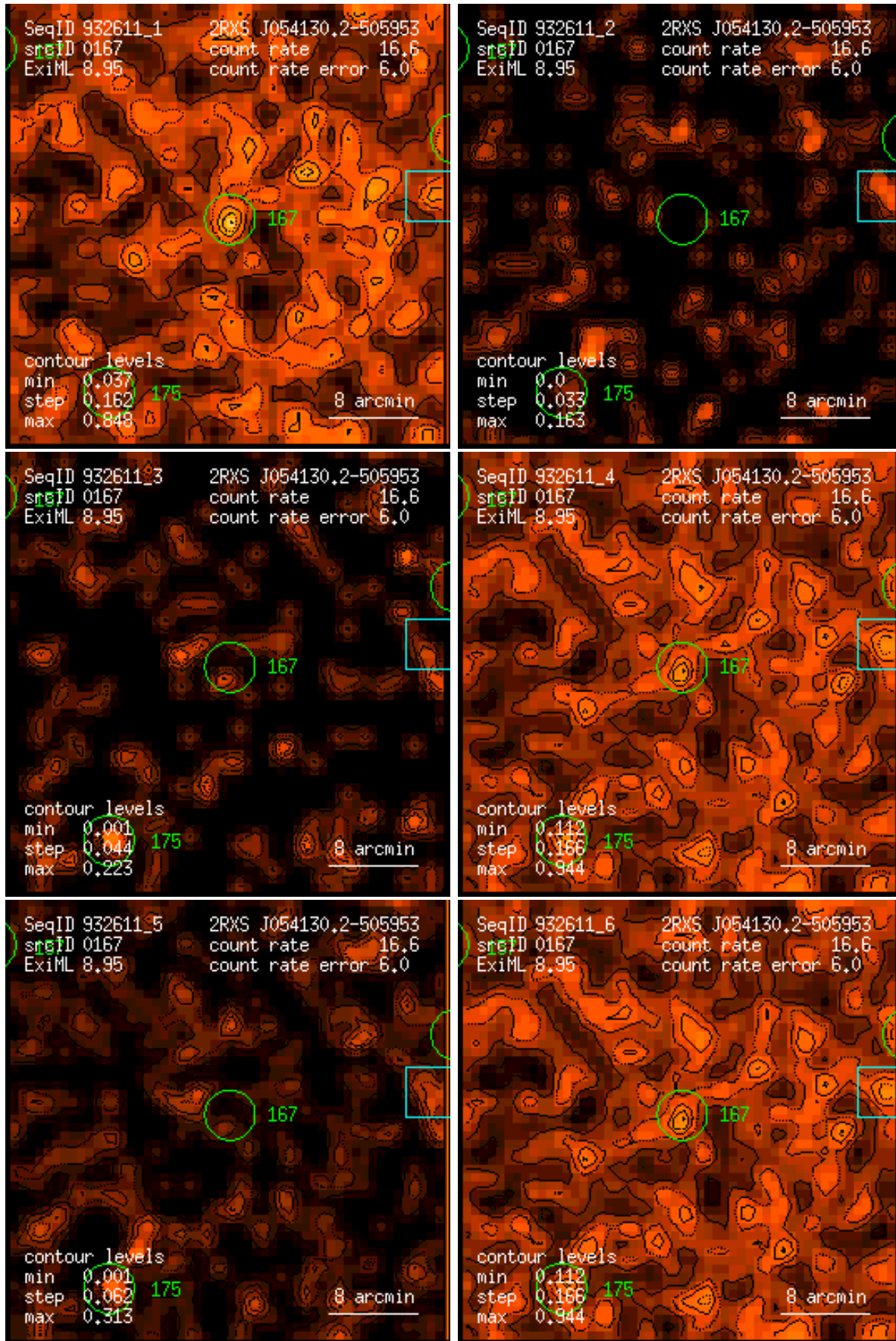
Figure 167: RASS 932611: detection 0167: band rate images, Gaussian filter: (1) PSPC channels 11 – 41, (2) 52 – 90, (3) 91 – 201, (4) 11 – 235, (5) 52 – 201, (6) 11 – 201. Broad band rates in counts/ks. Band rate contour levels in counts/ks/arcmin 2 .
