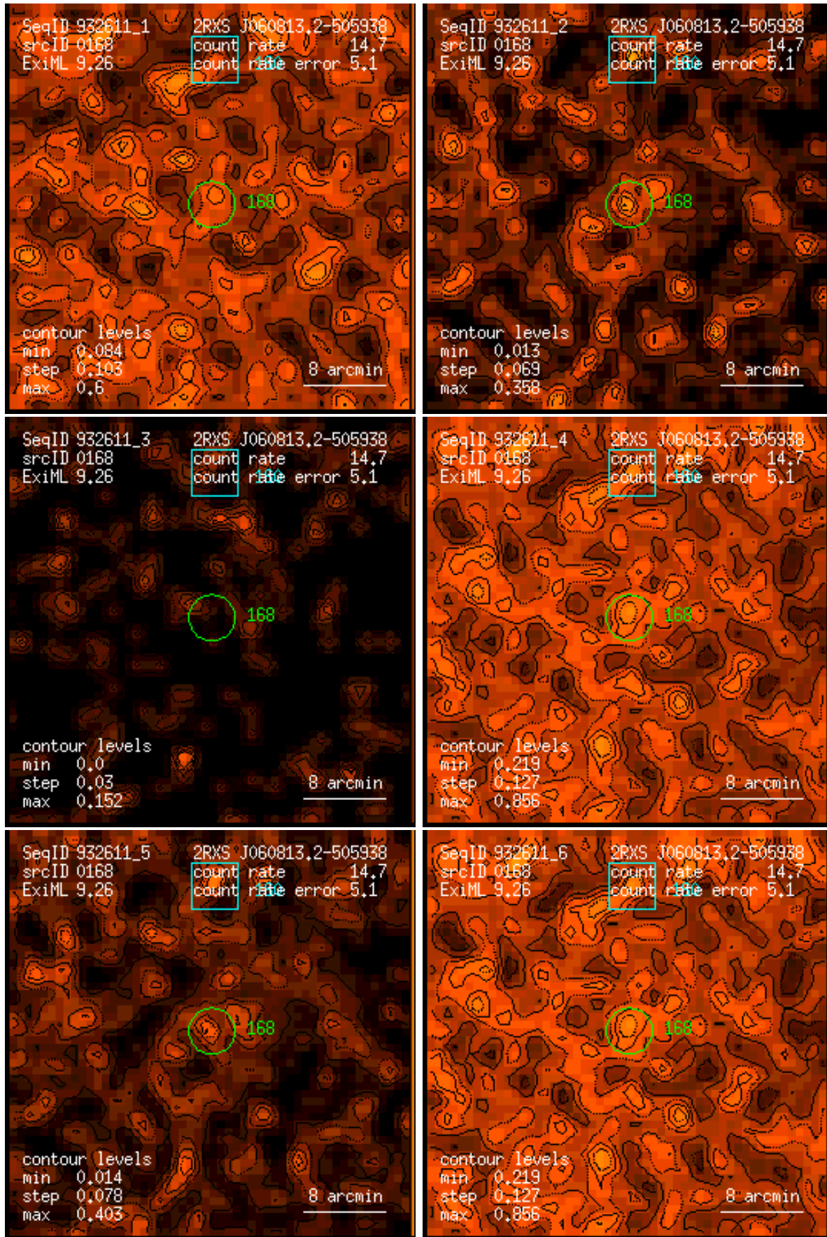
Figure 168: RASS 932611: detection 0168: band rate images, Gaussian filter: (1) PSPC channels 11 – 41, (2) 52 – 90, (3) 91 – 201, (4) 11 – 235, (5) 52 – 201, (6) 11 – 201. Broad band rates in counts/ks. Band rate contour levels in counts/ks/arcmin 2 .
