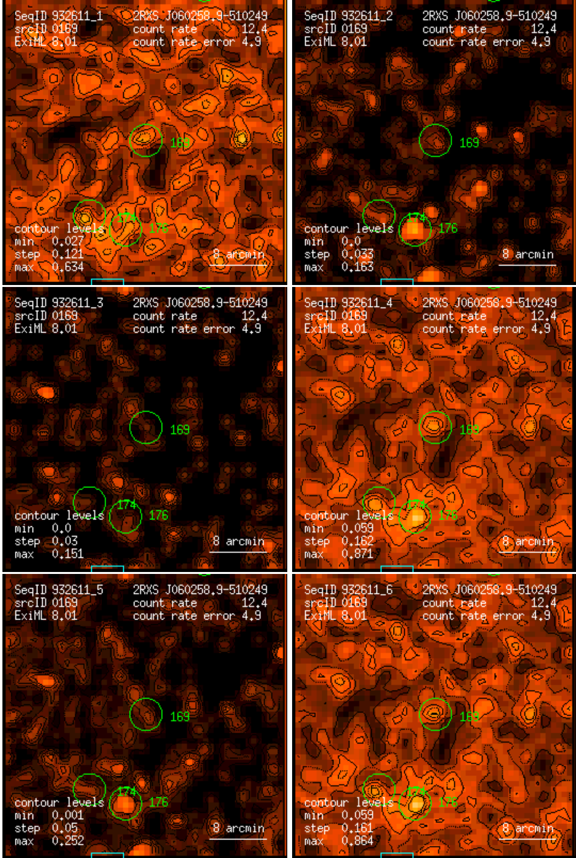
Figure 169: RASS 932611: detection 0169: band rate images, Gaussian filter: (1) PSPC channels 11 – 41, (2) 52 – 90, (3) 91 – 201, (4) 11 – 235, (5) 52 – 201, (6) 11 – 201. Broad band rates in counts/ks. Band rate contour levels in counts/ks/arcmin 2 .
