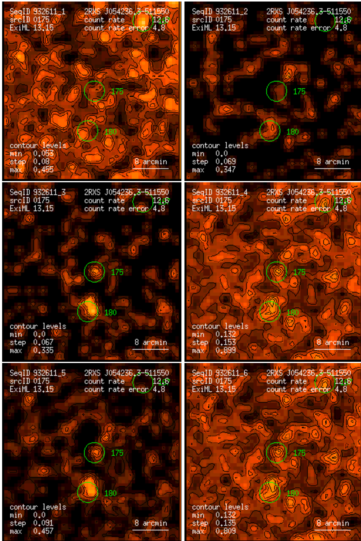
Figure 175: RASS 932611: detection 0175: band rate images, Gaussian filter: (1) PSPC channels 11 – 41, (2) 52 – 90, (3) 91 – 201, (4) 11 – 235, (5) 52 – 201, (6) 11 – 201. Broad band rates in counts/ks. Band rate contour levels in counts/ks/arcmin 2 .
