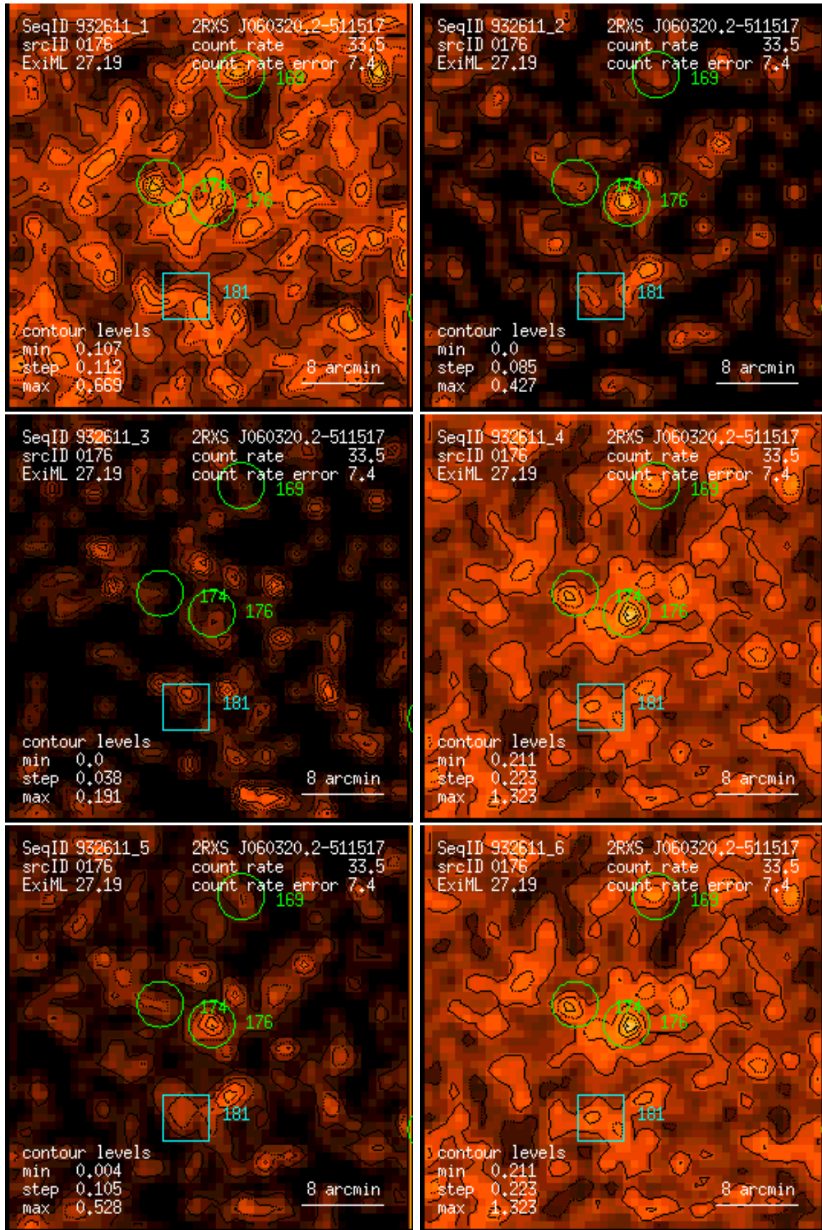
Figure 176: RASS 932611: detection 0176: band rate images, Gaussian filter: (1) PSPC channels 11 – 41, (2) 52 – 90, (3) 91 – 201, (4) 11 – 235, (5) 52 – 201, (6) 11 – 201. Broad band rates in counts/ks. Band rate contour levels in counts/ks/arcmin 2 .
