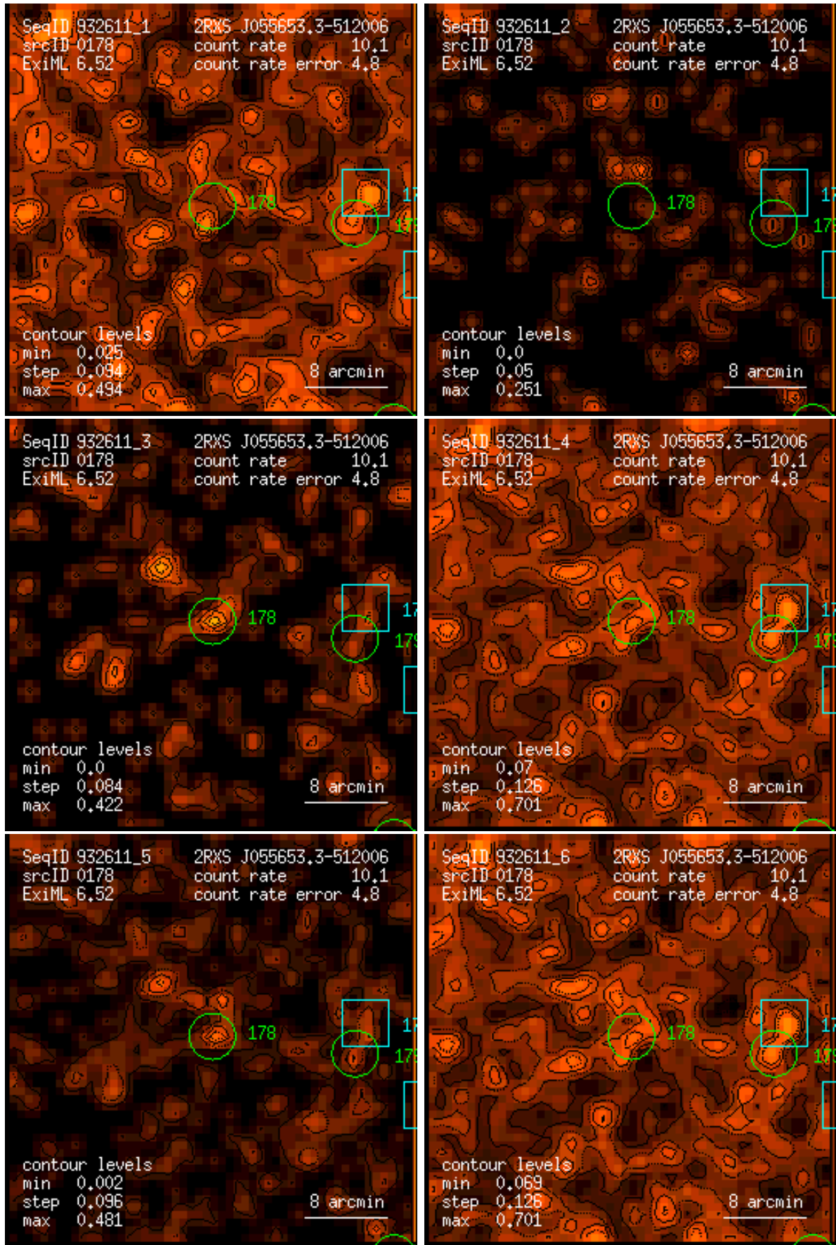
Figure 178: RASS 932611: detection 0178: band rate images, Gaussian filter: (1) PSPC channels 11 – 41, (2) 52 – 90, (3) 91 – 201, (4) 11 – 235, (5) 52 – 201, (6) 11 – 201. Broad band rates in counts/ks. Band rate contour levels in counts/ks/arcmin 2 .
