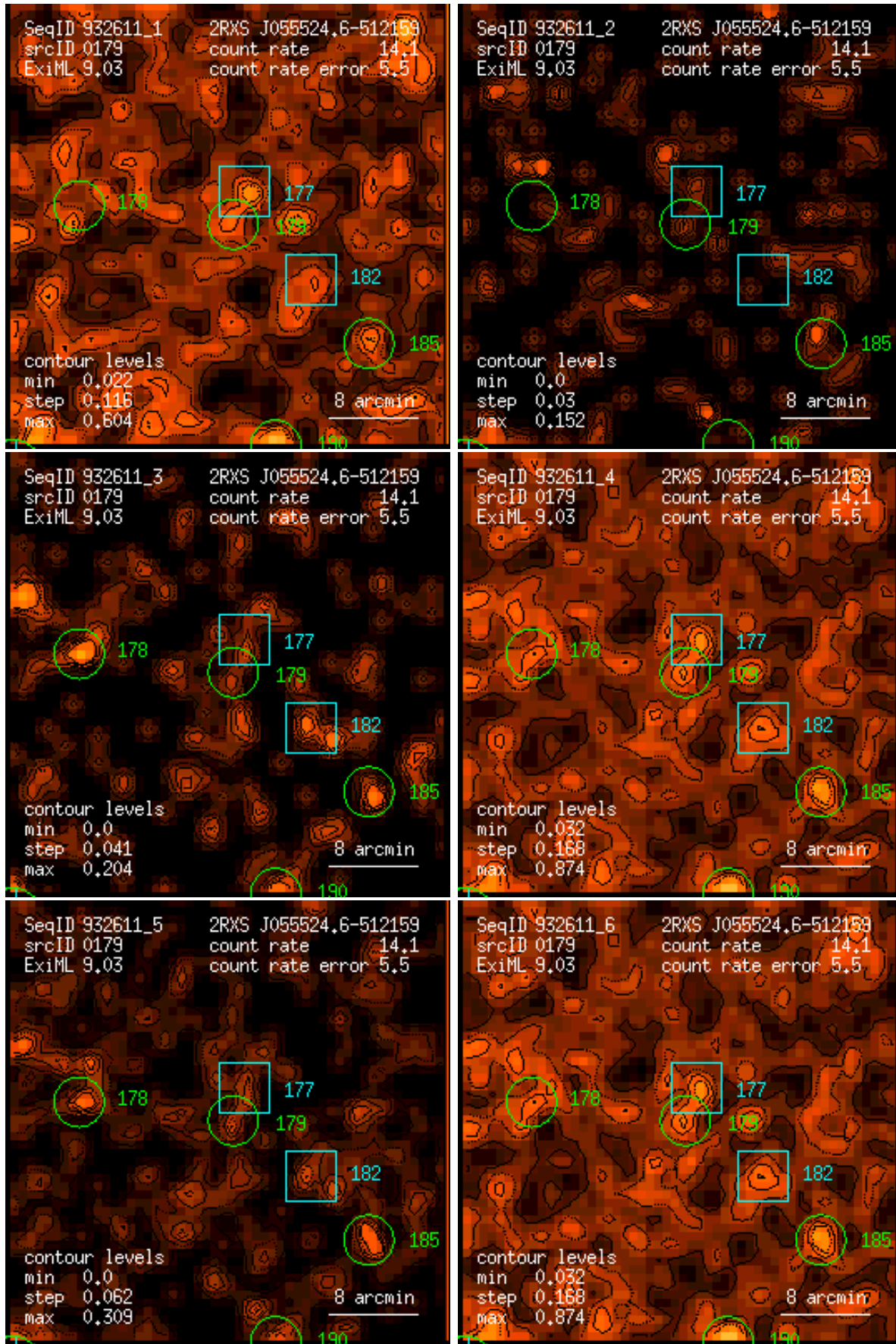
Figure 179: RASS 932611: detection 0179: band rate images, Gaussian filter: (1) PSPC channels 11 – 41, (2) 52 – 90, (3) 91 – 201, (4) 11 – 235, (5) 52 – 201, (6) 11 – 201. Broad band rates in counts/ks. Band rate contour levels in counts/ks/arcmin 2 .
