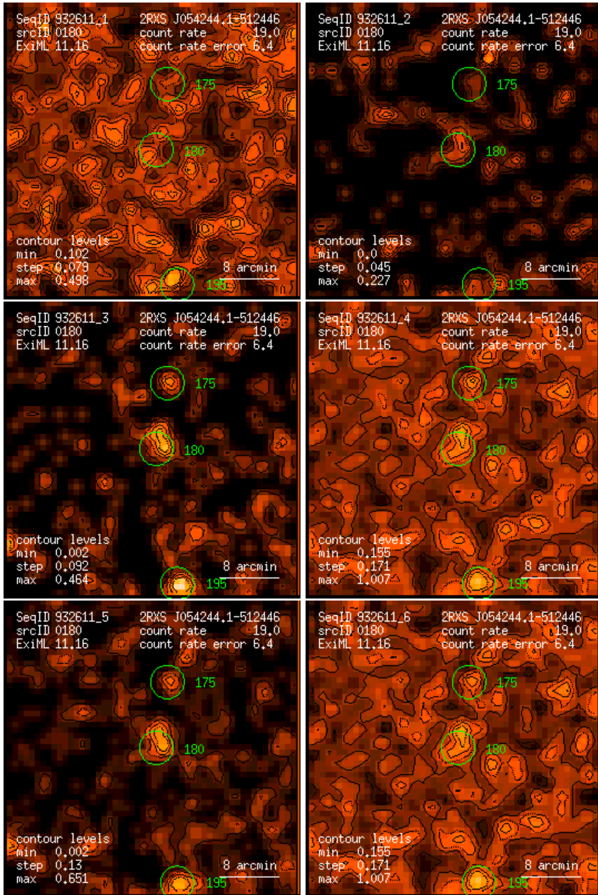
Figure 180: RASS 932611: detection 0180: band rate images, Gaussian filter: (1) PSPC channels 11 – 41, (2) 52 – 90, (3) 91 – 201, (4) 11 – 235, (5) 52 – 201, (6) 11 – 201. Broad band rates in counts/ks. Band rate contour levels in counts/ks/arcmin 2 .
